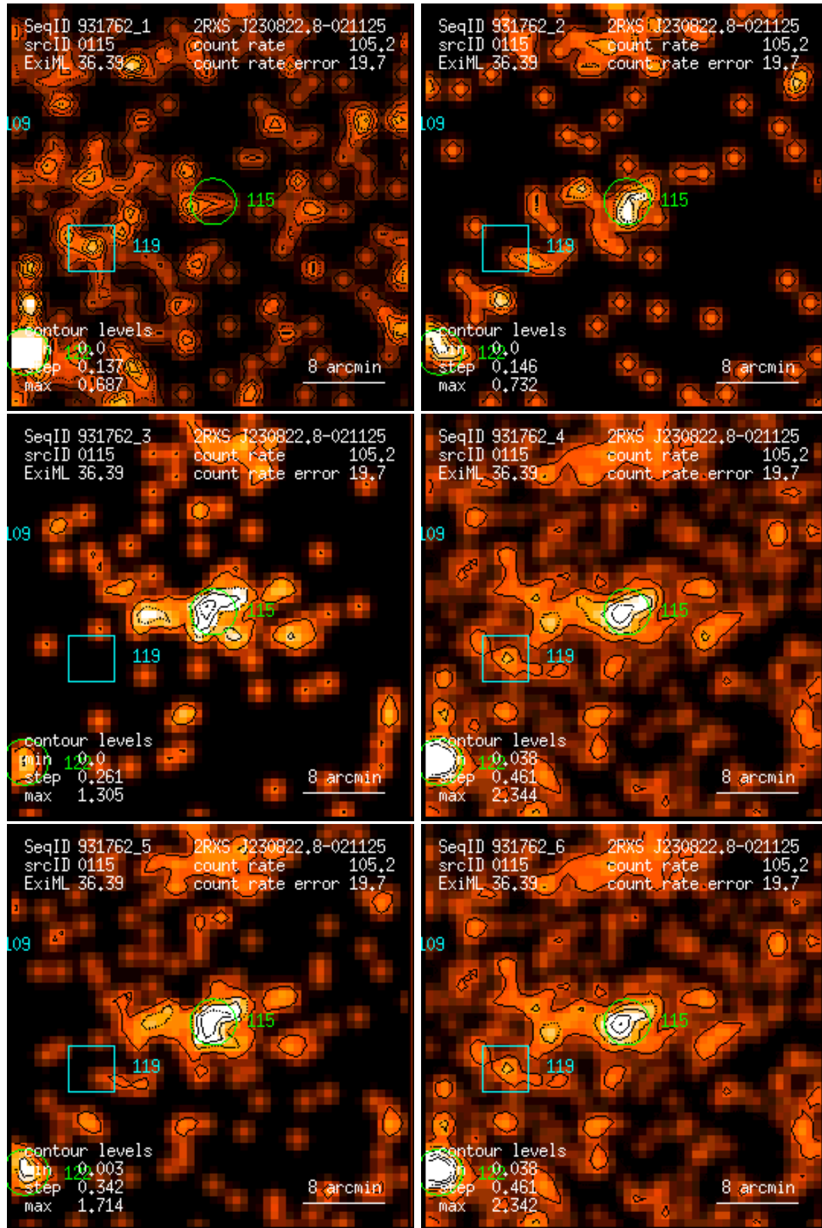
Figure 115: RASS 931762: detection 0115: band rate images, Gaussian filter: (1) PSPC channels 11 – 41, (2) 52 – 90, (3) 91 – 201, (4) 11 – 235, (5) 52 – 201, (6) 11 – 201. Broad band rates in counts/ks. Band rate contour levels in counts/ks/arcmin 2 .
