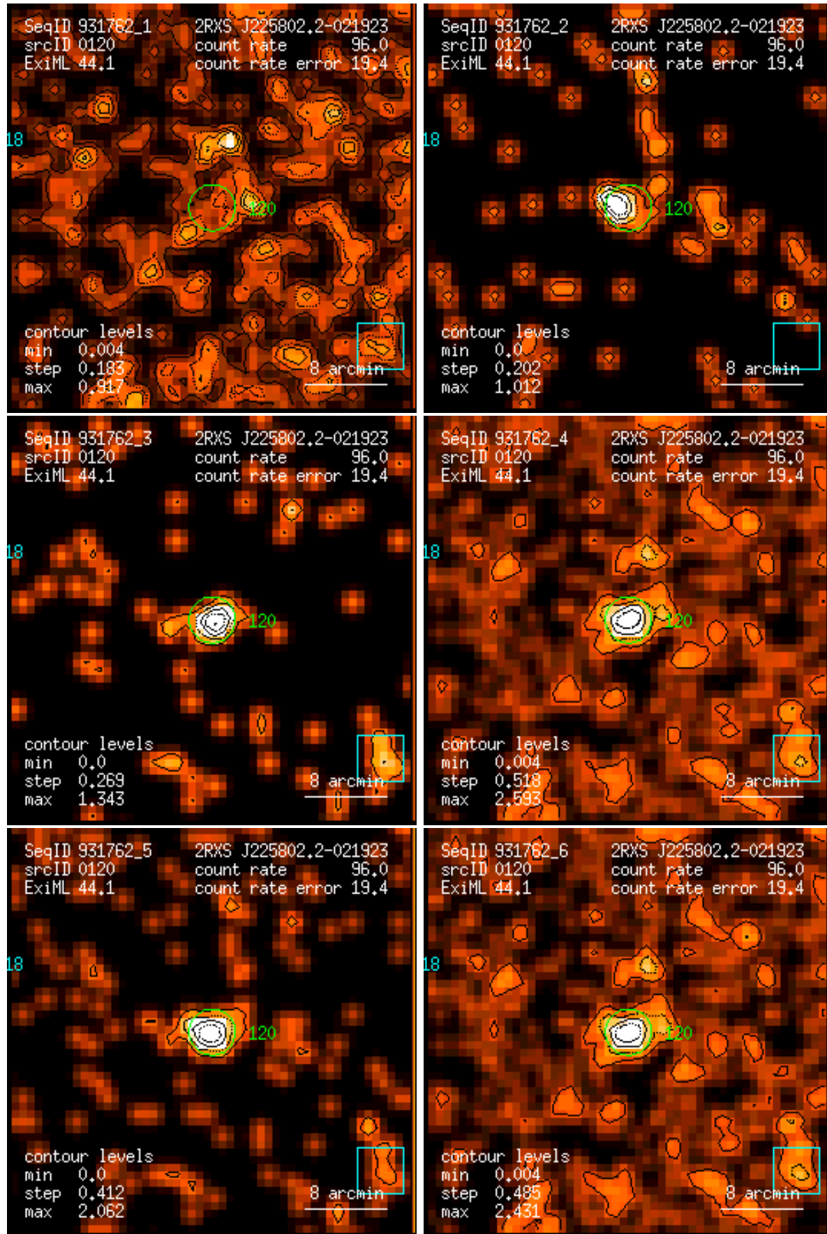
Figure 120: RASS 931762: detection 0120: band rate images, Gaussian filter: (1) PSPC channels 11 – 41, (2) 52 – 90, (3) 91 – 201, (4) 11 – 235, (5) 52 – 201, (6) 11 – 201. Broad band rates in counts/ks. Band rate contour levels in counts/ks/arcmin 2 .
