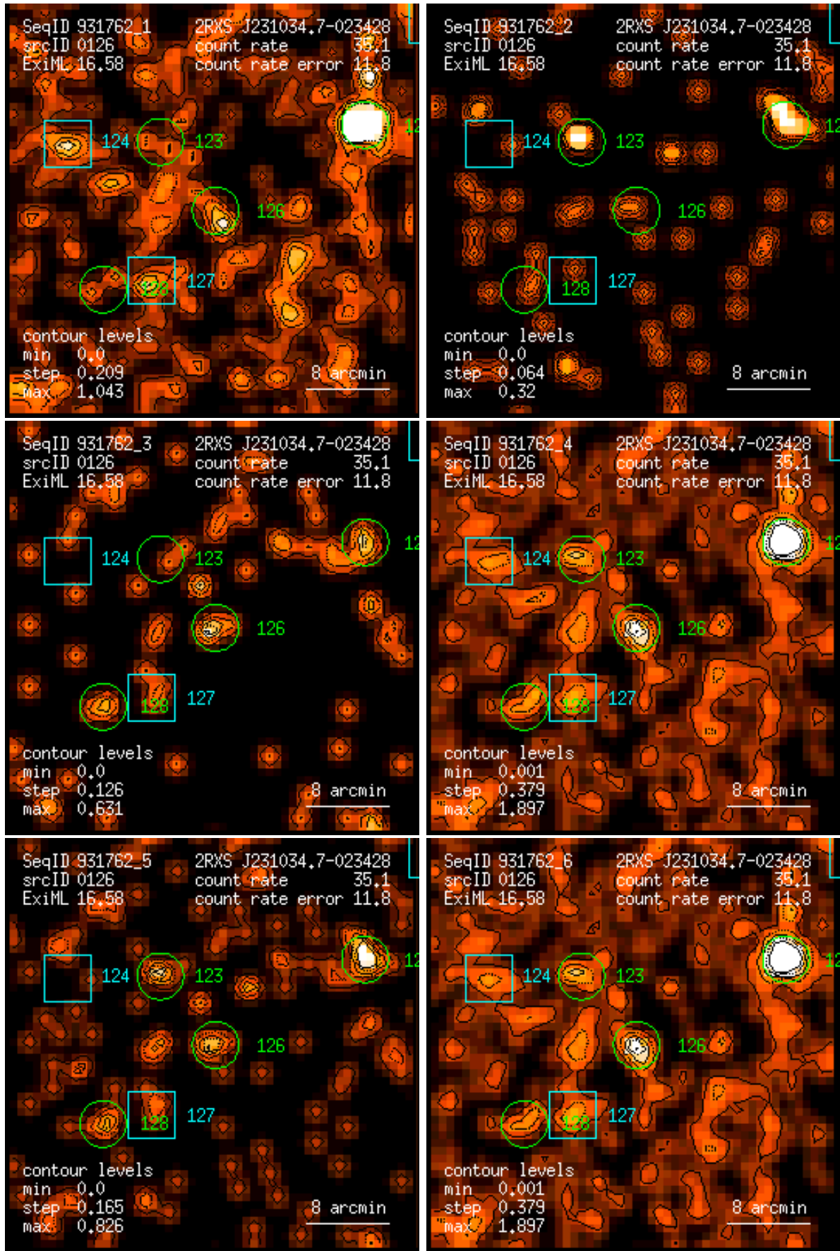
Figure 126: RASS 931762: detection 0126: band rate images, Gaussian filter: (1) PSPC channels 11 – 41, (2) 52 – 90, (3) 91 – 201, (4) 11 – 235, (5) 52 – 201, (6) 11 – 201. Broad band rates in counts/ks. Band rate contour levels in counts/ks/arcmin 2 .
