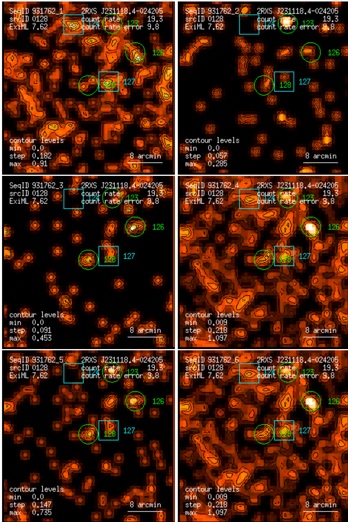
Figure 128: RASS 931762: detection 0128: band rate images, Gaussian filter: (1) PSPC channels 11 – 41, (2) 52 – 90, (3) 91 – 201, (4) 11 – 235, (5) 52 – 201, (6) 11 – 201. Broad band rates in counts/ks. Band rate contour levels in counts/ks/arcmin 2 .
