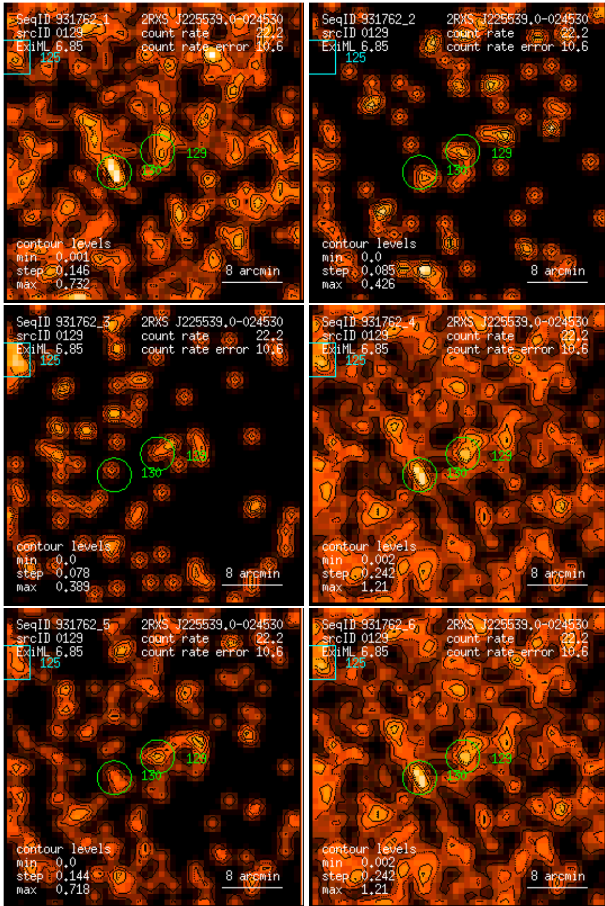
Figure 129: RASS 931762: detection 0129: band rate images, Gaussian filter: (1) PSPC channels 11 – 41, (2) 52 – 90, (3) 91 – 201, (4) 11 – 235, (5) 52 – 201, (6) 11 – 201. Broad band rates in counts/ks. Band rate contour levels in counts/ks/arcmin 2 .
