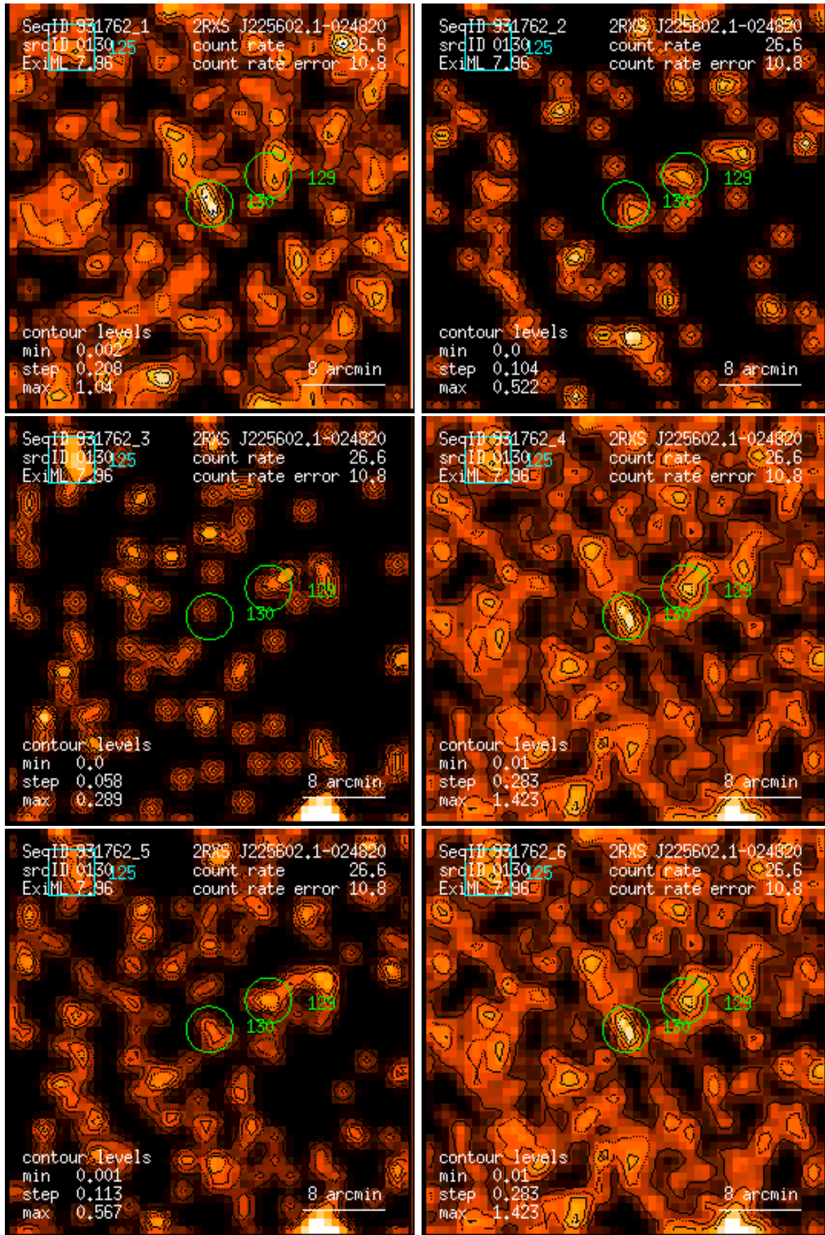
Figure 130: RASS 931762: detection 0130: band rate images, Gaussian filter: (1) PSPC channels 11 – 41, (2) 52 – 90, (3) 91 – 201, (4) 11 – 235, (5) 52 – 201, (6) 11 – 201. Broad band rates in counts/ks. Band rate contour levels in counts/ks/arcmin 2 .
