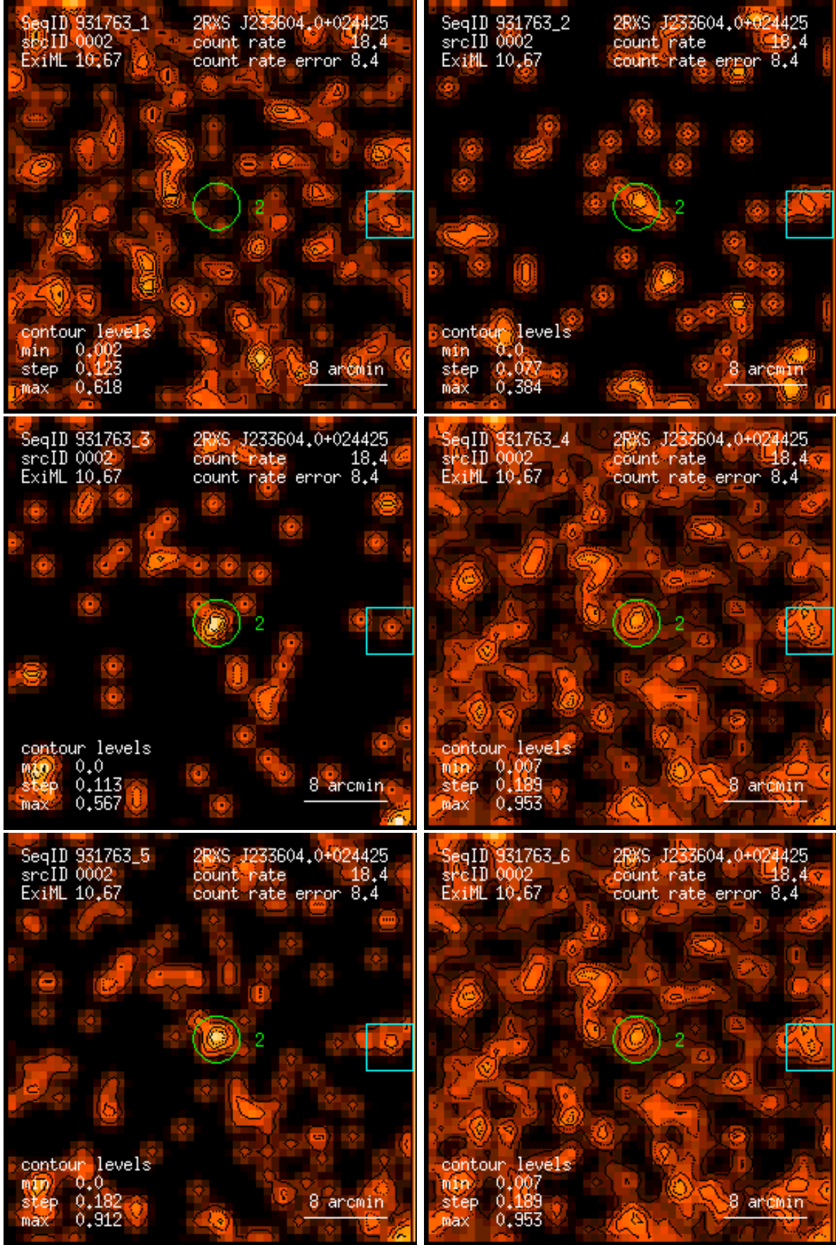
Figure 2: RASS 931763: detection 0002: band rate images, Gaussian filter: (1) PSPC channels 11 – 41, (2) 52 – 90, (3) 91 – 201, (4) 11 – 235, (5) 52 – 201, (6) 11 – 201. Broad band rates in counts/ks. Band rate contour levels in counts/ks/arcmin 2 .
