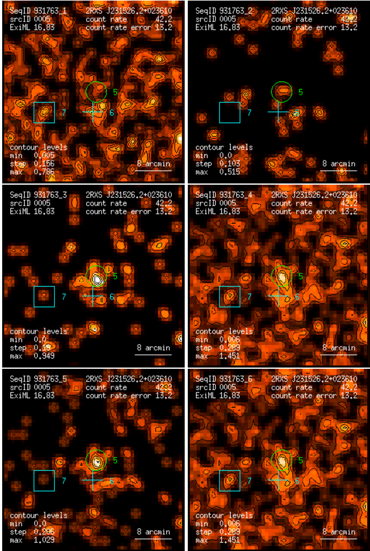
Figure 5: RASS 931763: detection 0005: band rate images, Gaussian filter: (1) PSPC channels 11 – 41, (2) 52 – 90, (3) 91 – 201, (4) 11 – 235, (5) 52 – 201, (6) 11 – 201. Broad band rates in counts/ks. Band rate contour levels in counts/ks/arcmin 2 .
