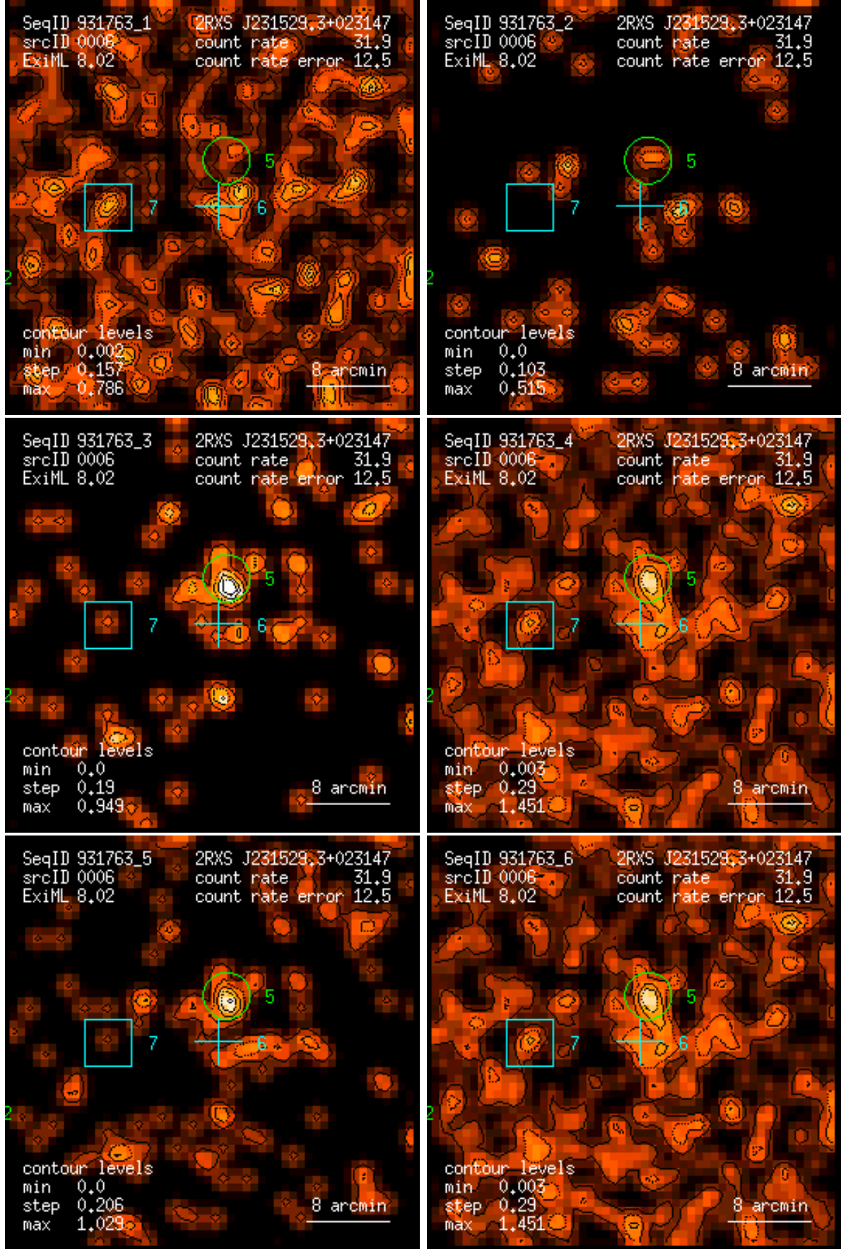
Figure 6: RASS 931763: detection 0006: band rate images, Gaussian filter: (1) PSPC channels 11 – 41, (2) 52 – 90, (3) 91 – 201, (4) 11 – 235, (5) 52 – 201, (6) 11 – 201. Broad band rates in counts/ks. Band rate contour levels in counts/ks/arcmin 2 .
