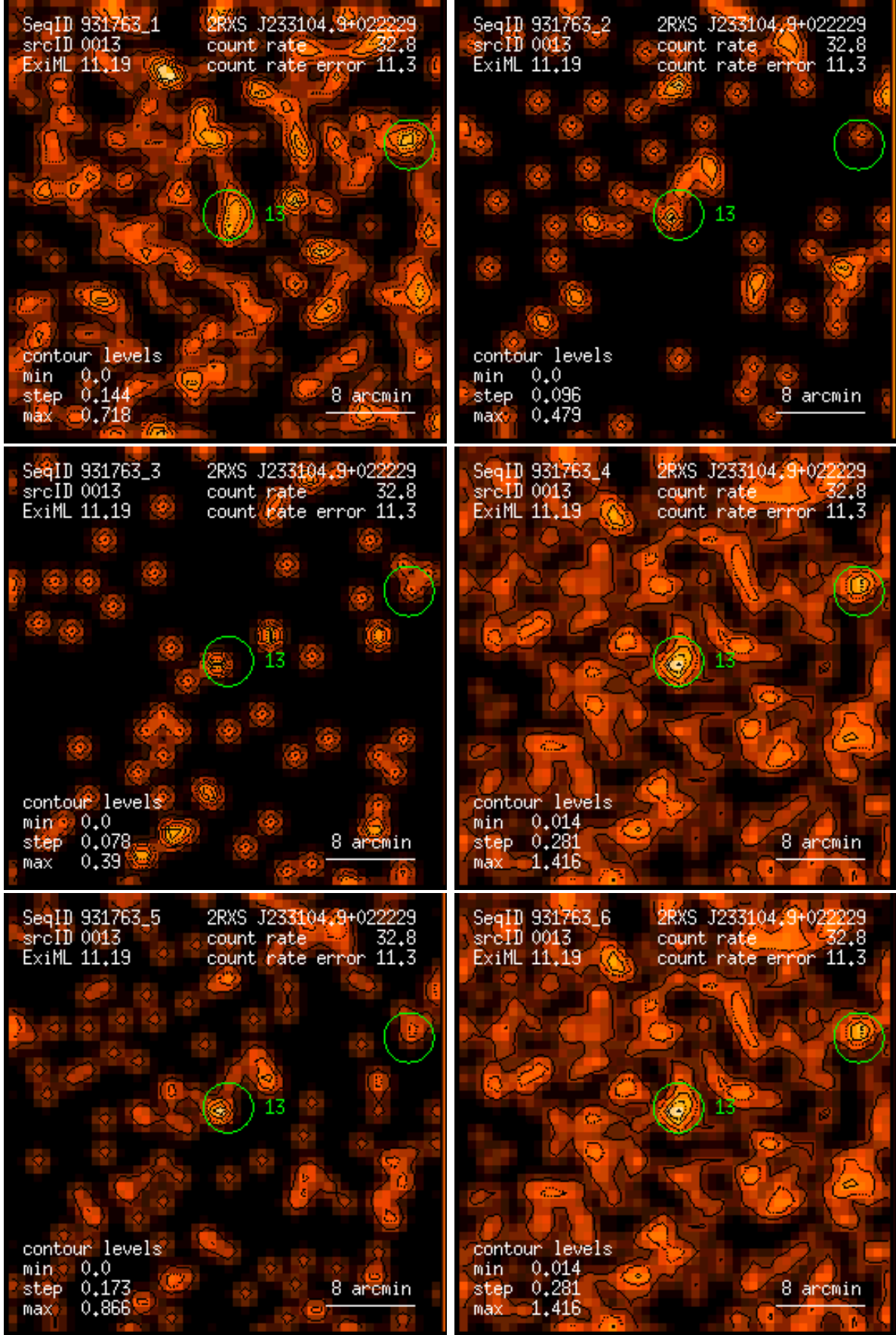
Figure 13: RASS 931763: detection 0013: band rate images, Gaussian filter: (1) PSPC channels 11 – 41, (2) 52 – 90, (3) 91 – 201, (4) 11 – 235, (5) 52 – 201, (6) 11 – 201. Broad band rates in counts/ks. Band rate contour levels in counts/ks/arcmin 2 .
