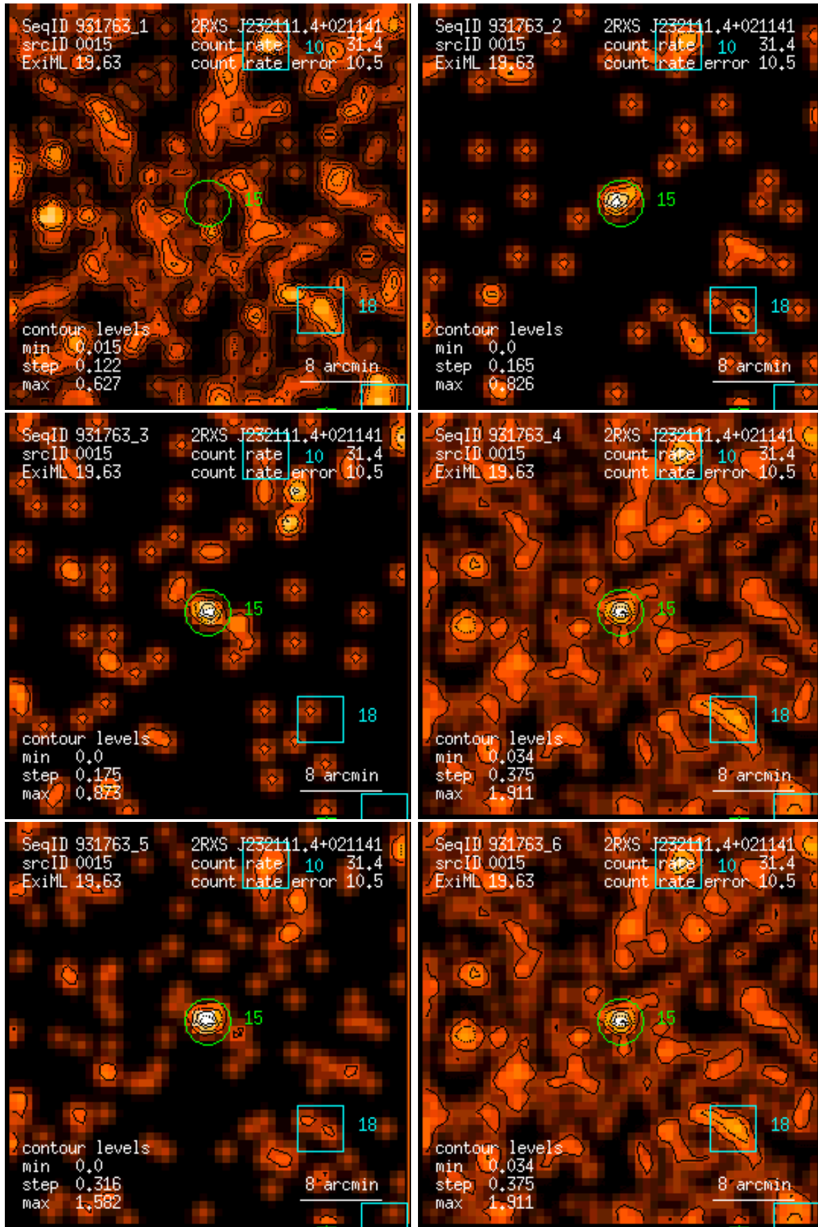
Figure 15: RASS 931763: detection 0015: band rate images, Gaussian filter: (1) PSPC channels 11 – 41, (2) 52 – 90, (3) 91 – 201, (4) 11 – 235, (5) 52 – 201, (6) 11 – 201. Broad band rates in counts/ks. Band rate contour levels in counts/ks/arcmin 2 .
