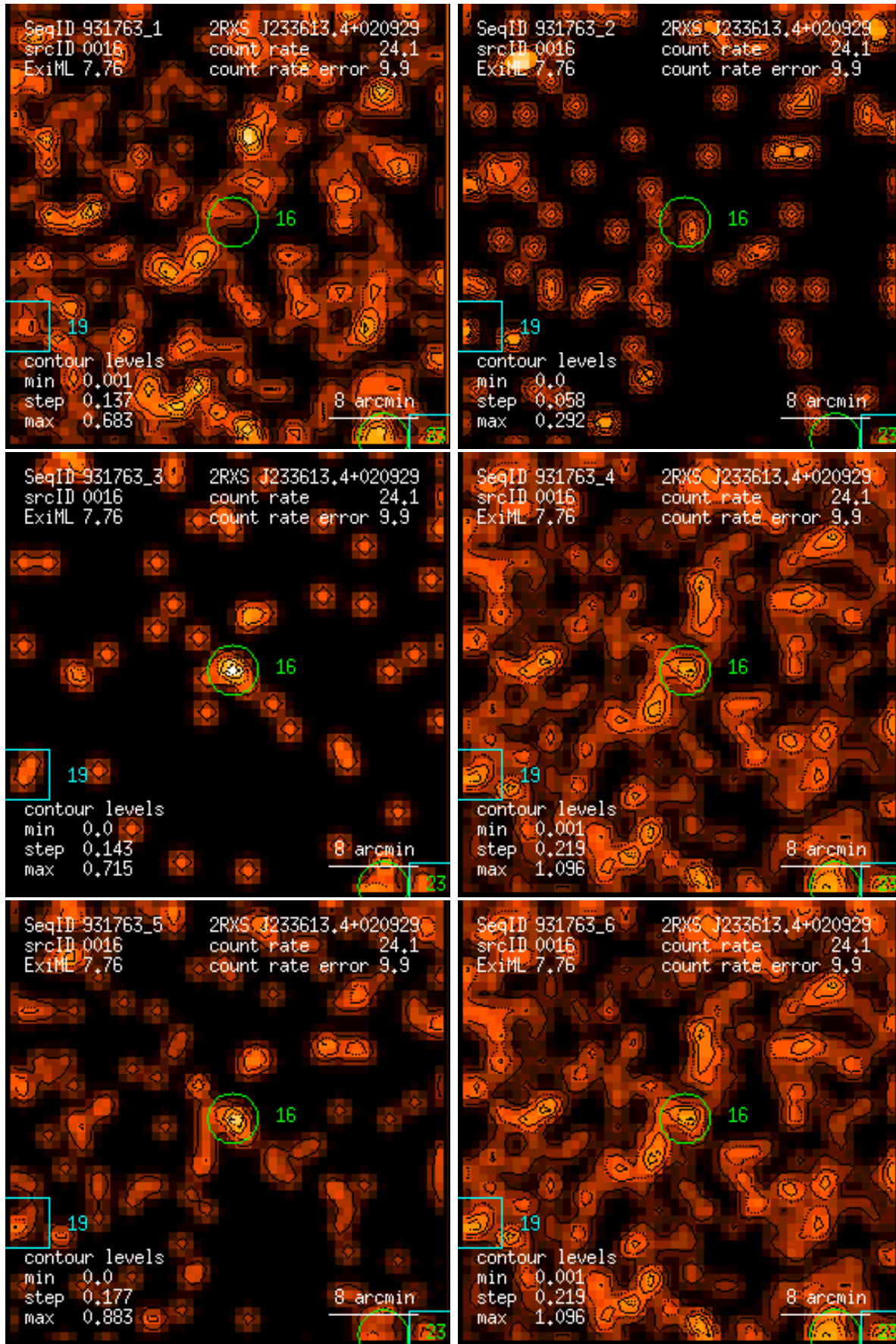
Figure 16: RASS 931763: detection 0016: band rate images, Gaussian filter: (1) PSPC channels 11 – 41, (2) 52 – 90, (3) 91 – 201, (4) 11 – 235, (5) 52 – 201, (6) 11 – 201. Broad band rates in counts/ks. Band rate contour levels in counts/ks/arcmin 2 .
