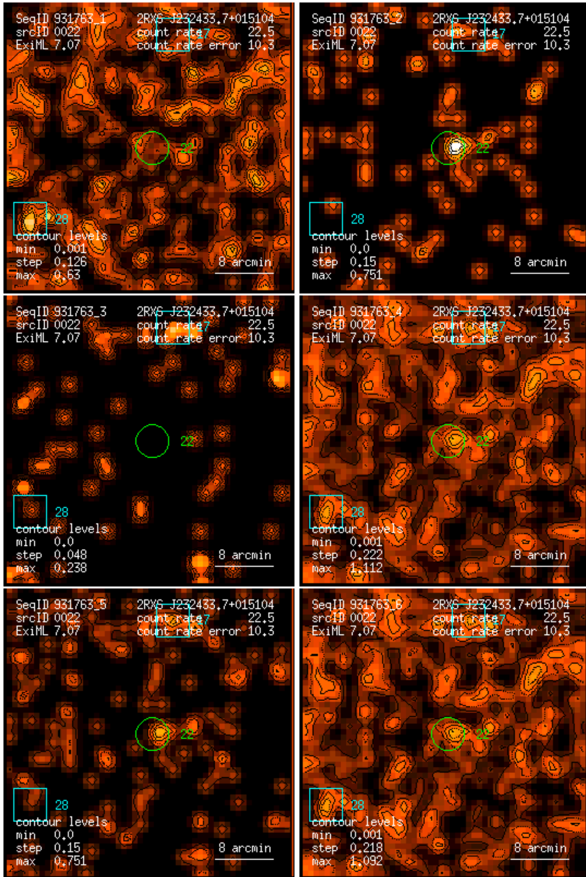
Figure 22: RASS 931763: detection 0022: band rate images, Gaussian filter: (1) PSPC channels 11 – 41, (2) 52 – 90, (3) 91 – 201, (4) 11 – 235, (5) 52 – 201, (6) 11 – 201. Broad band rates in counts/ks. Band rate contour levels in counts/ks/arcmin 2 .
