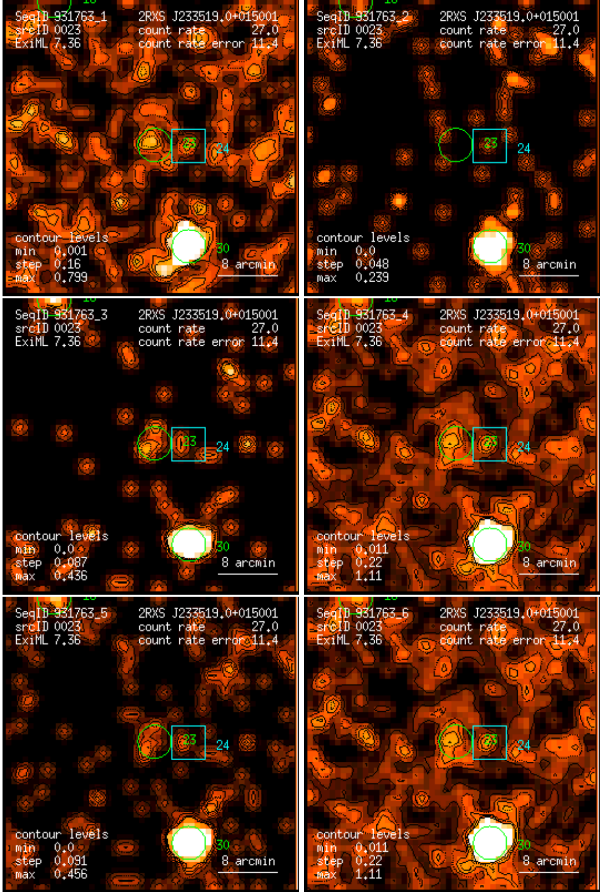
Figure 23: RASS 931763: detection 0023: band rate images, Gaussian filter: (1) PSPC channels 11 – 41, (2) 52 – 90, (3) 91 – 201, (4) 11 – 235, (5) 52 – 201, (6) 11 – 201. Broad band rates in counts/ks. Band rate contour levels in counts/ks/arcmin 2 .
