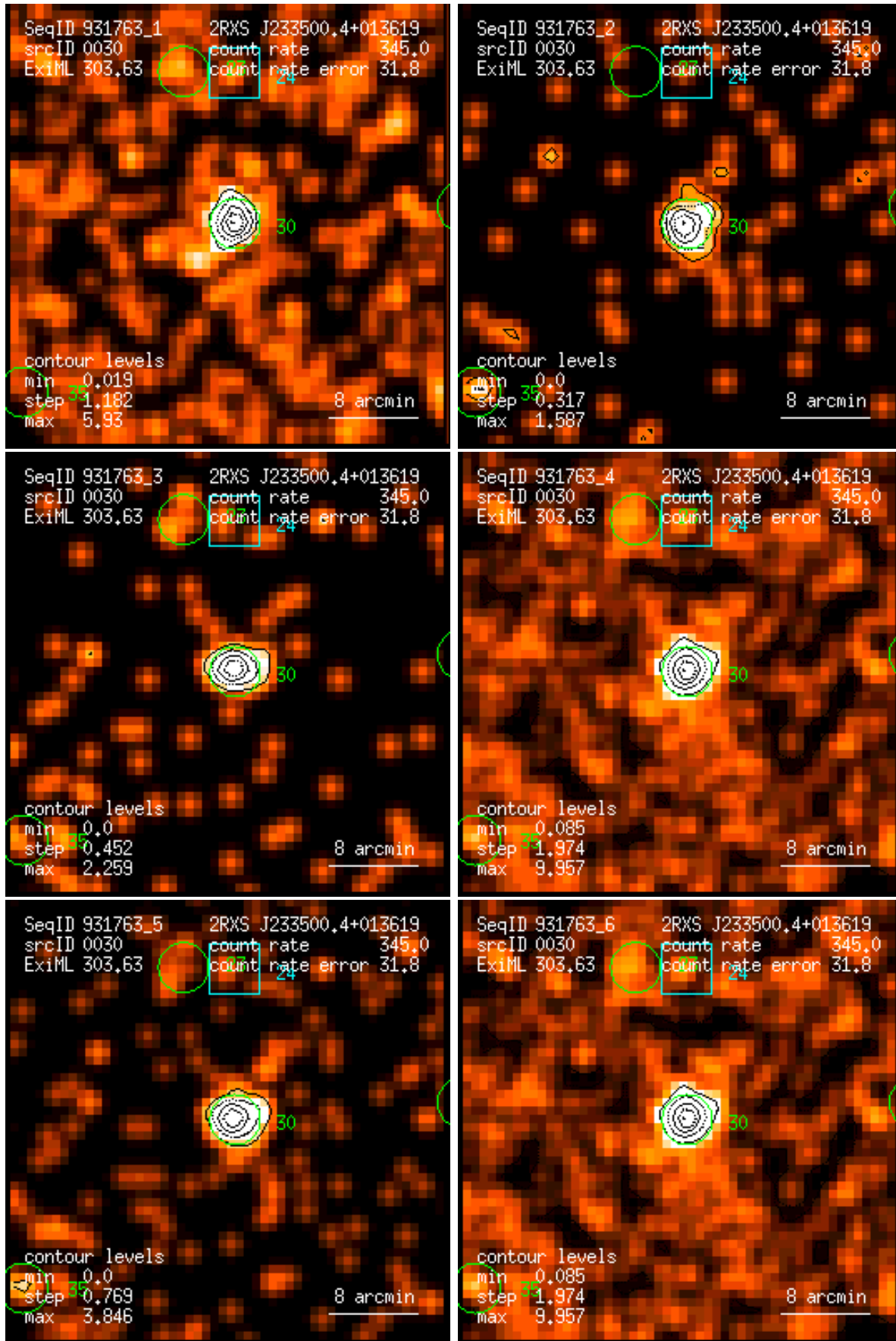
Figure 30: RASS 931763: detection 0030: band rate images, Gaussian filter: (1) PSPC channels 11 – 41, (2) 52 – 90, (3) 91 – 201, (4) 11 – 235, (5) 52 – 201, (6) 11 – 201. Broad band rates in counts/ks. Band rate contour levels in counts/ks/arcmin 2 .
