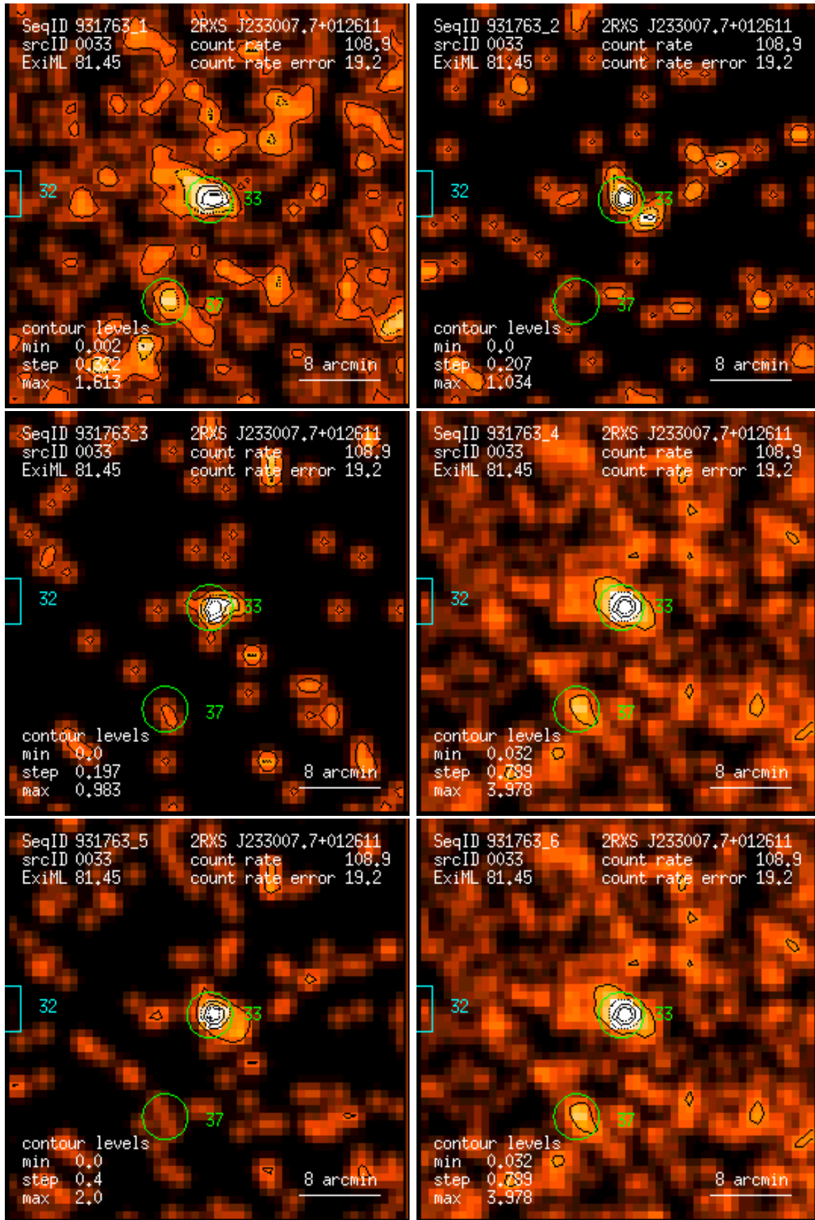
Figure 33: RASS 931763: detection 0033: band rate images, Gaussian filter: (1) PSPC channels 11 – 41, (2) 52 – 90, (3) 91 – 201, (4) 11 – 235, (5) 52 – 201, (6) 11 – 201. Broad band rates in counts/ks. Band rate contour levels in counts/ks/arcmin 2 .
