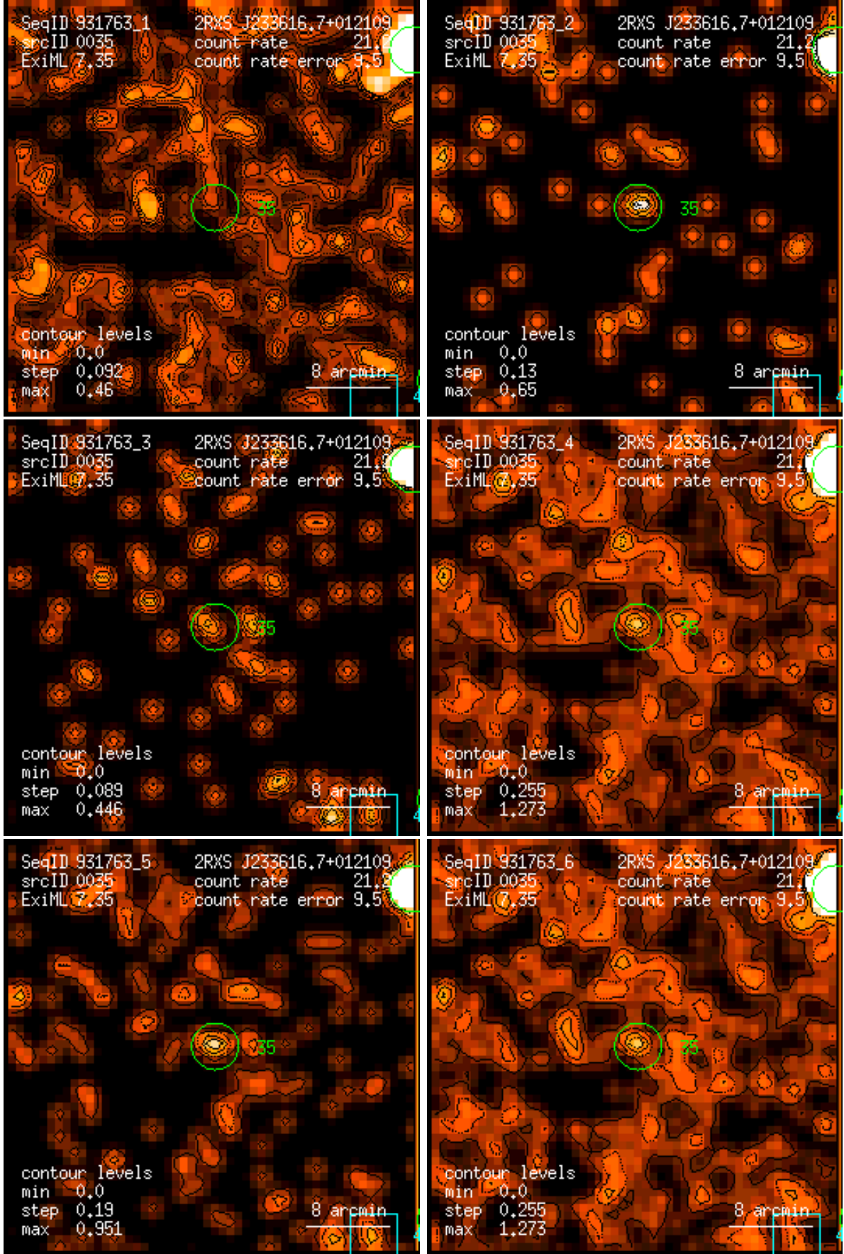
Figure 35: RASS 931763: detection 0035: band rate images, Gaussian filter: (1) PSPC channels 11 – 41, (2) 52 – 90, (3) 91 – 201, (4) 11 – 235, (5) 52 – 201, (6) 11 – 201. Broad band rates in counts/ks. Band rate contour levels in counts/ks/arcmin 2 .
