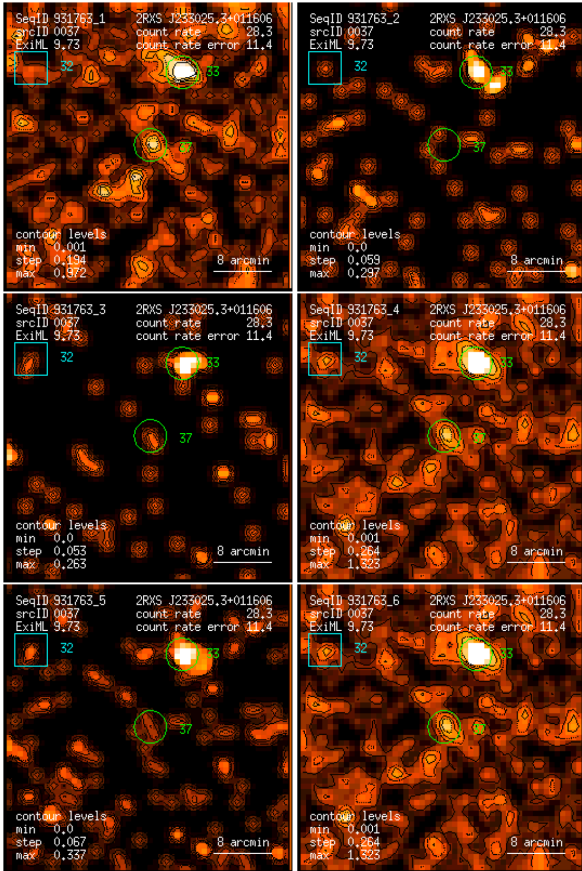
Figure 37: RASS 931763: detection 0037: band rate images, Gaussian filter: (1) PSPC channels 11 – 41, (2) 52 – 90, (3) 91 – 201, (4) 11 – 235, (5) 52 – 201, (6) 11 – 201. Broad band rates in counts/ks. Band rate contour levels in counts/ks/arcmin 2 .
