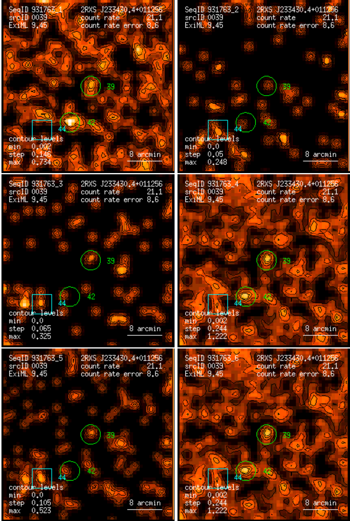
Figure 39: RASS 931763: detection 0039: band rate images, Gaussian filter: (1) PSPC channels 11 – 41, (2) 52 – 90, (3) 91 – 201, (4) 11 – 235, (5) 52 – 201, (6) 11 – 201. Broad band rates in counts/ks. Band rate contour levels in counts/ks/arcmin 2 .
