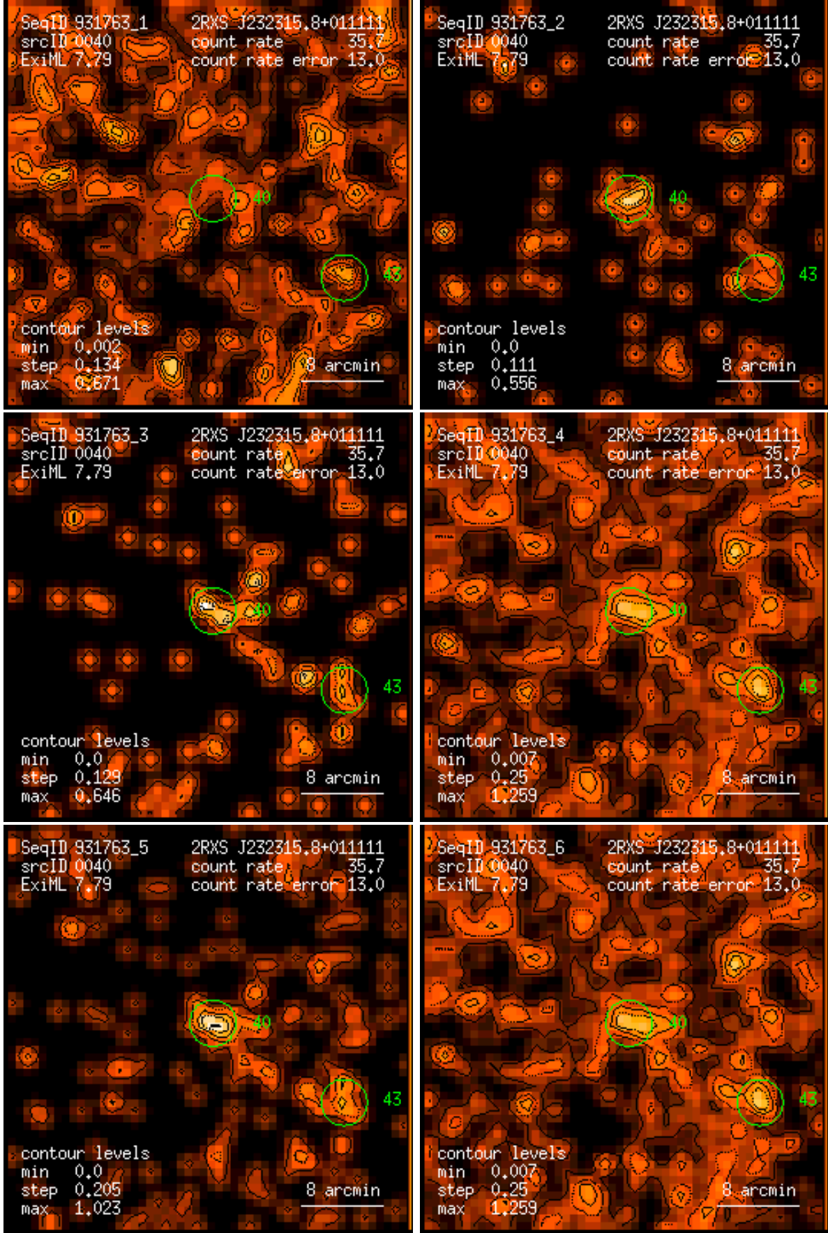
Figure 40: RASS 931763: detection 0040: band rate images, Gaussian filter: (1) PSPC channels 11 – 41, (2) 52 – 90, (3) 91 – 201, (4) 11 – 235, (5) 52 – 201, (6) 11 – 201. Broad band rates in counts/ks. Band rate contour levels in counts/ks/arcmin 2 .
