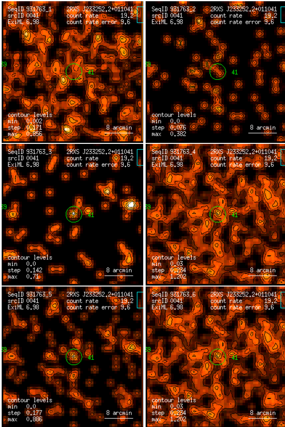
Figure 41: RASS 931763: detection 0041: band rate images, Gaussian filter: (1) PSPC channels 11 – 41, (2) 52 – 90, (3) 91 – 201, (4) 11 – 235, (5) 52 – 201, (6) 11 – 201. Broad band rates in counts/ks. Band rate contour levels in counts/ks/arcmin 2 .
