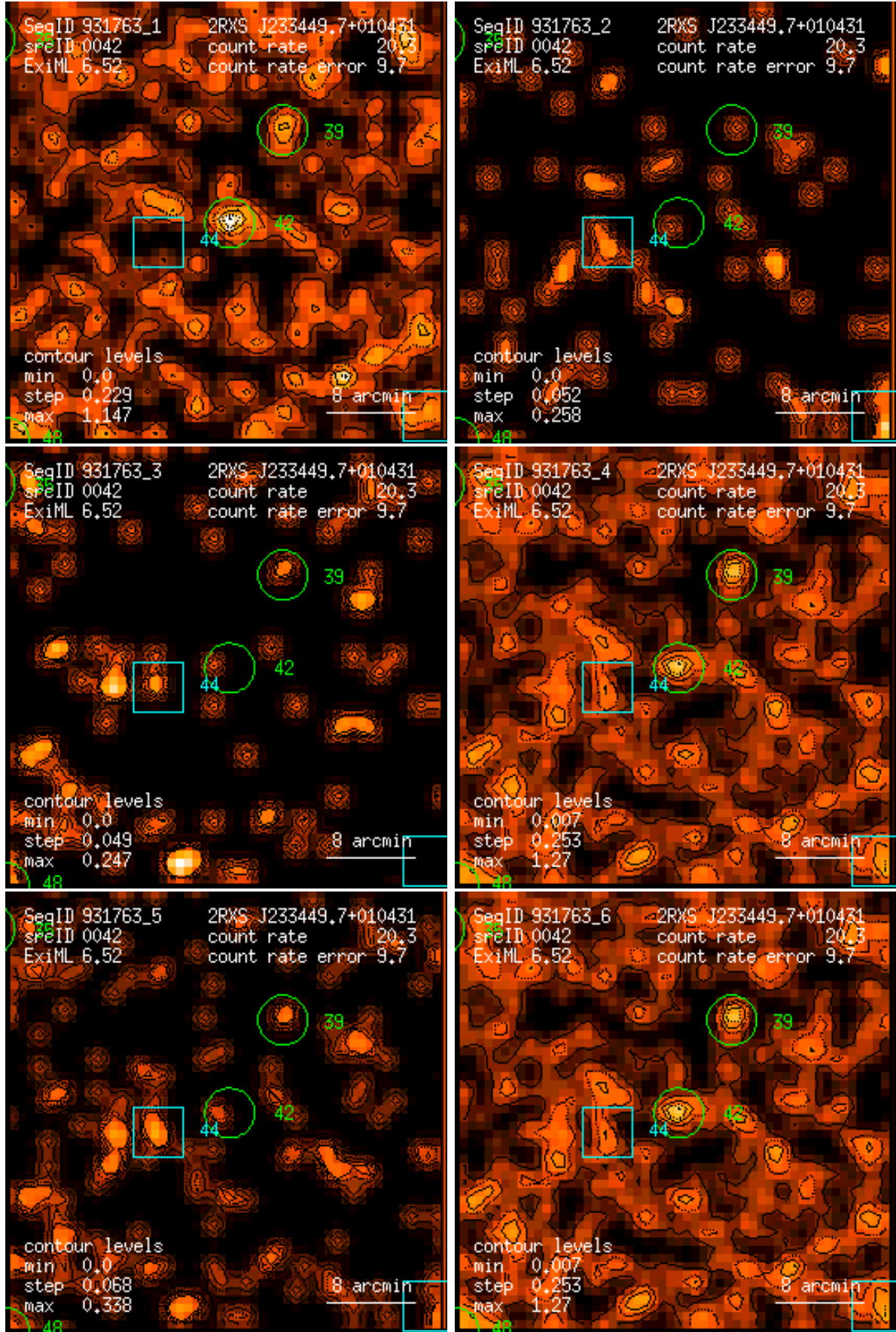
Figure 42: RASS 931763: detection 0042: band rate images, Gaussian filter: (1) PSPC channels 11 – 41, (2) 52 – 90, (3) 91 – 201, (4) 11 – 235, (5) 52 – 201, (6) 11 – 201. Broad band rates in counts/ks. Band rate contour levels in counts/ks/arcmin 2 .
