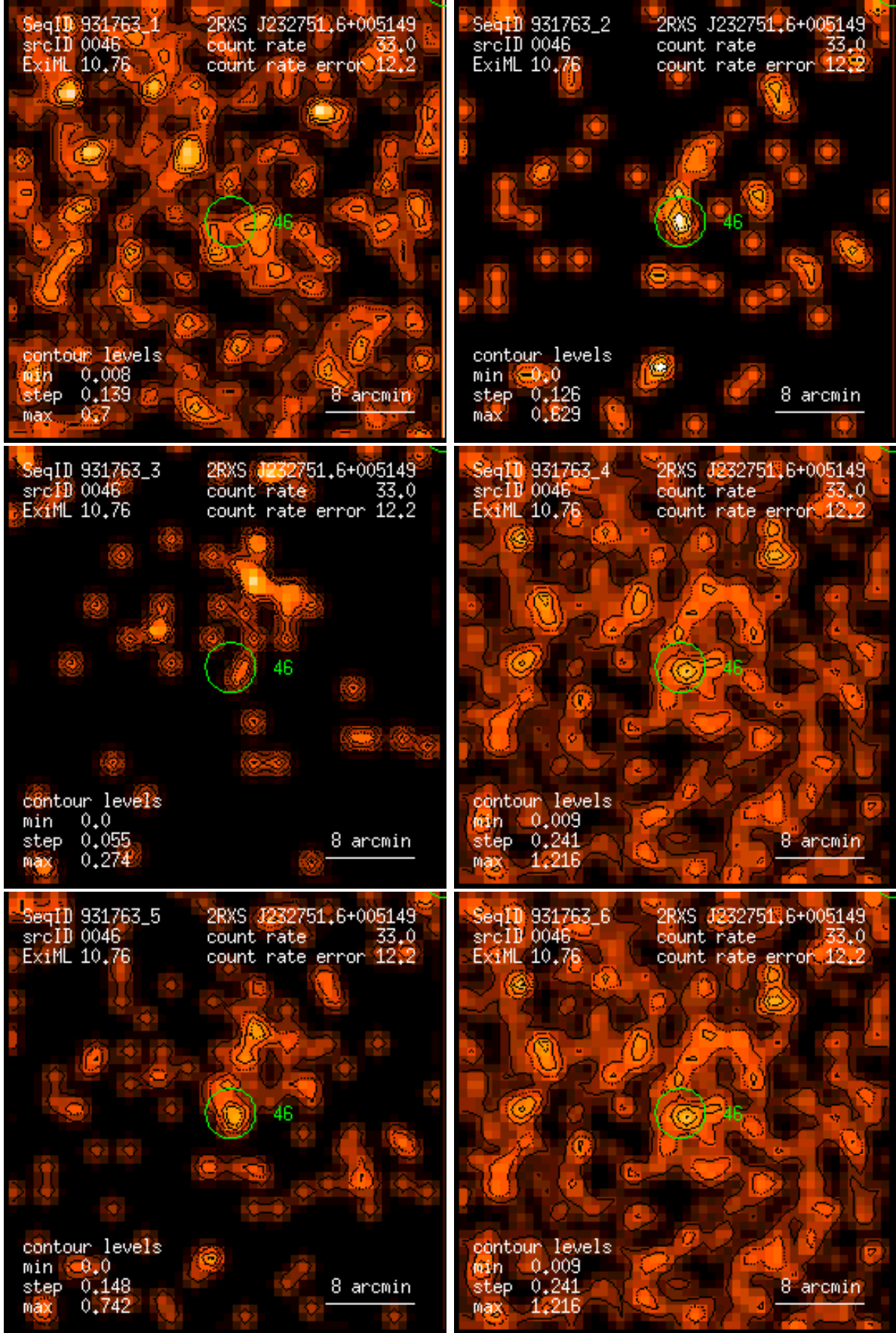
Figure 46: RASS 931763: detection 0046: band rate images, Gaussian filter: (1) PSPC channels 11 – 41, (2) 52 – 90, (3) 91 – 201, (4) 11 – 235, (5) 52 – 201, (6) 11 – 201. Broad band rates in counts/ks. Band rate contour levels in counts/ks/arcmin 2 .
