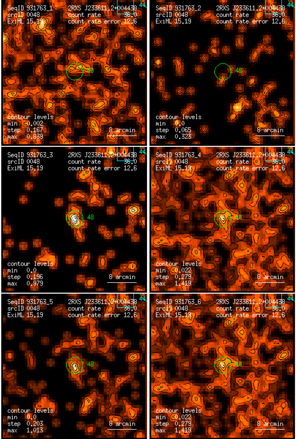
Figure 48: RASS 931763: detection 0048: band rate images, Gaussian filter: (1) PSPC channels 11 – 41, (2) 52 – 90, (3) 91 – 201, (4) 11 – 235, (5) 52 – 201, (6) 11 – 201. Broad band rates in counts/ks. Band rate contour levels in counts/ks/arcmin 2 .
