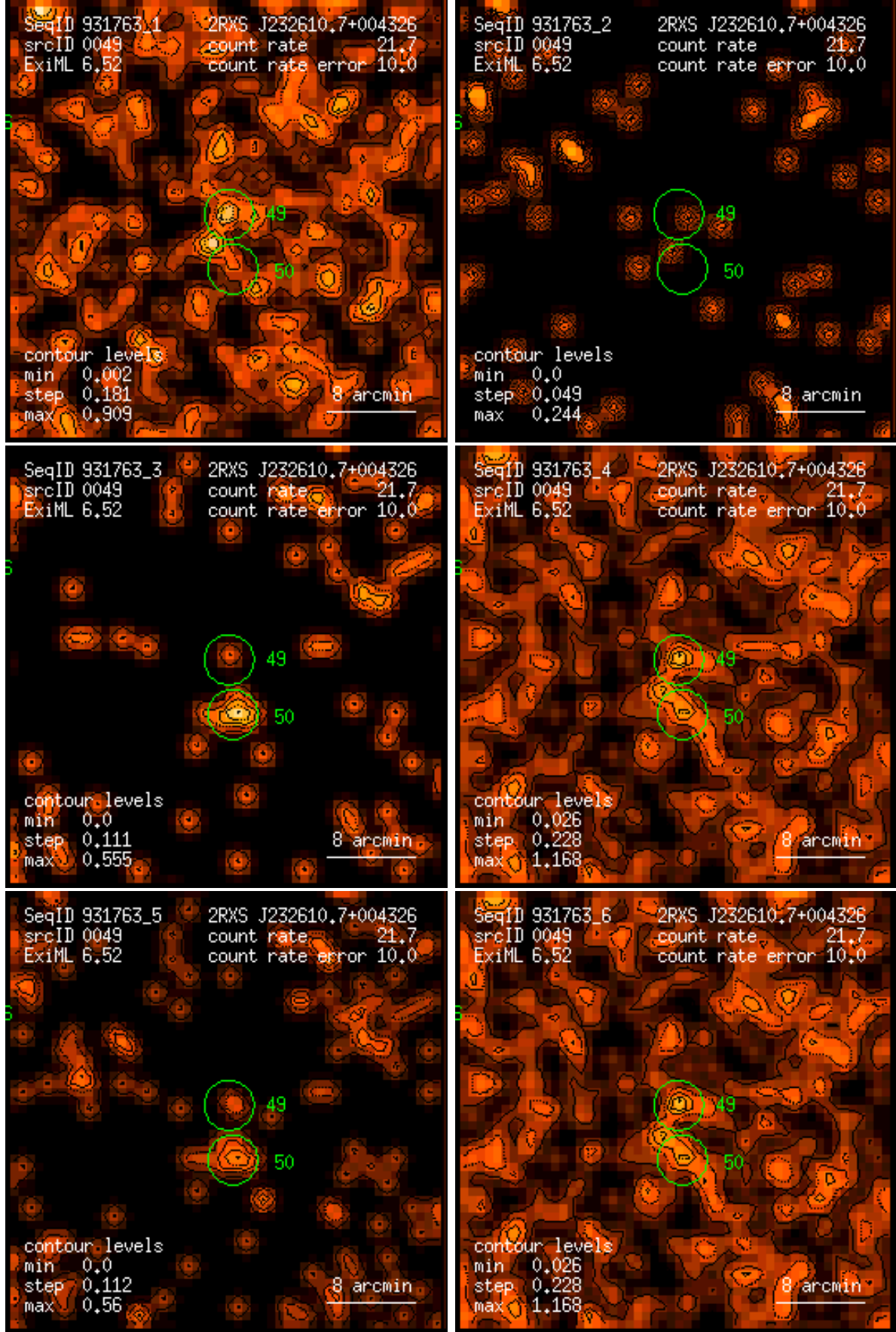
Figure 49: RASS 931763: detection 0049: band rate images, Gaussian filter: (1) PSPC channels 11 – 41, (2) 52 – 90, (3) 91 – 201, (4) 11 – 235, (5) 52 – 201, (6) 11 – 201. Broad band rates in counts/ks. Band rate contour levels in counts/ks/arcmin 2 .
