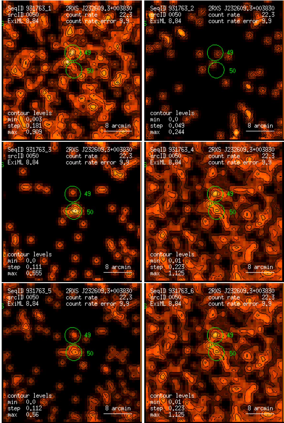
Figure 50: RASS 931763: detection 0050: band rate images, Gaussian filter: (1) PSPC channels 11 – 41, (2) 52 – 90, (3) 91 – 201, (4) 11 – 235, (5) 52 – 201, (6) 11 – 201. Broad band rates in counts/ks. Band rate contour levels in counts/ks/arcmin 2 .
