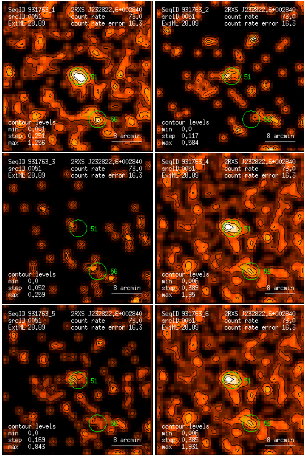
Figure 51: RASS 931763: detection 0051: band rate images, Gaussian filter: (1) PSPC channels 11 – 41, (2) 52 – 90, (3) 91 – 201, (4) 11 – 235, (5) 52 – 201, (6) 11 – 201. Broad band rates in counts/ks. Band rate contour levels in counts/ks/arcmin 2 .
