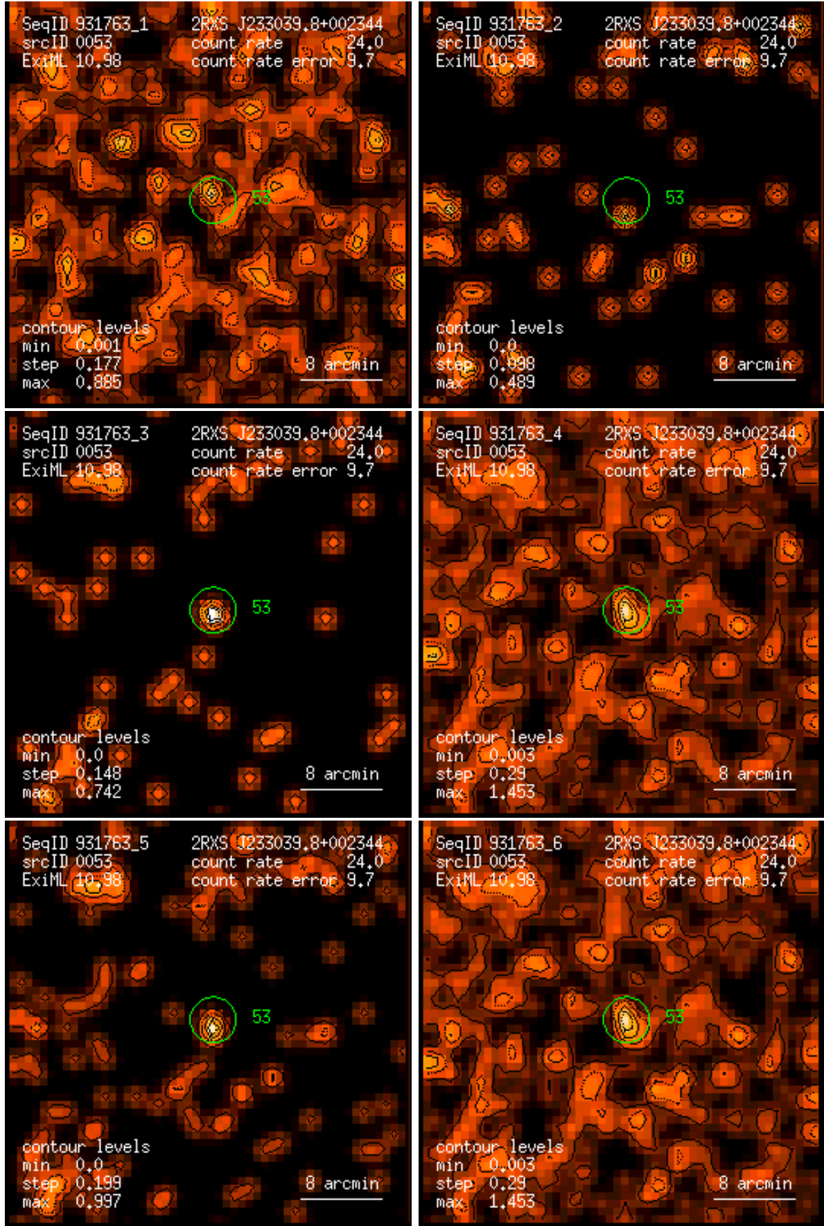
Figure 53: RASS 931763: detection 0053: band rate images, Gaussian filter: (1) PSPC channels 11 – 41, (2) 52 – 90, (3) 91 – 201, (4) 11 – 235, (5) 52 – 201, (6) 11 – 201. Broad band rates in counts/ks. Band rate contour levels in counts/ks/arcmin 2 .
