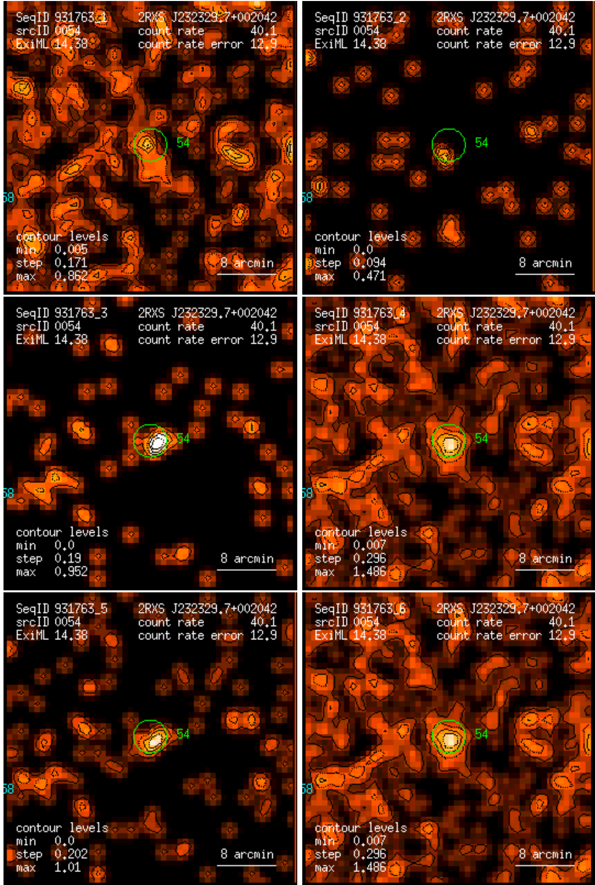
Figure 54: RASS 931763: detection 0054: band rate images, Gaussian filter: (1) PSPC channels 11 – 41, (2) 52 – 90, (3) 91 – 201, (4) 11 – 235, (5) 52 – 201, (6) 11 – 201. Broad band rates in counts/ks. Band rate contour levels in counts/ks/arcmin 2 .
