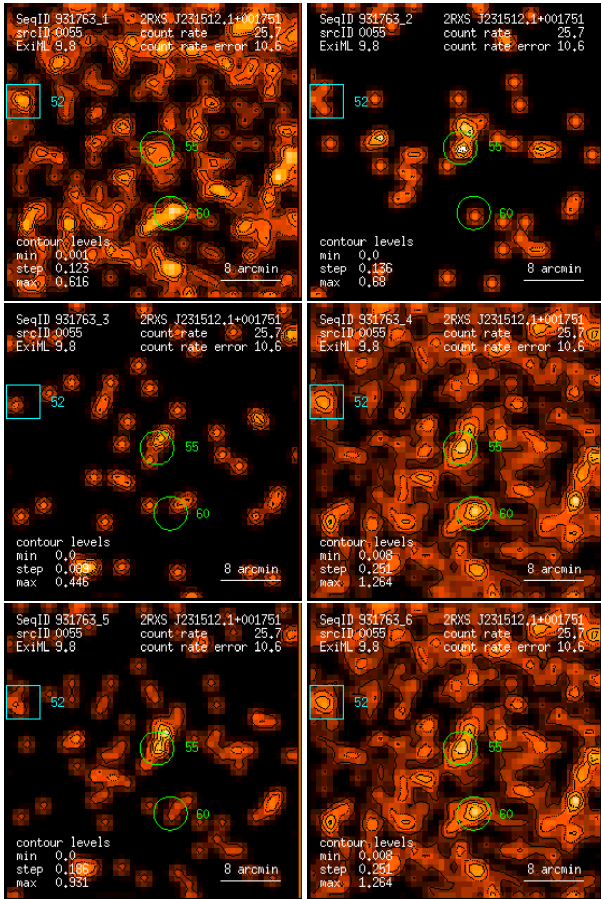
Figure 55: RASS 931763: detection 0055: band rate images, Gaussian filter: (1) PSPC channels 11 – 41, (2) 52 – 90, (3) 91 – 201, (4) 11 – 235, (5) 52 – 201, (6) 11 – 201. Broad band rates in counts/ks. Band rate contour levels in counts/ks/arcmin 2 .
