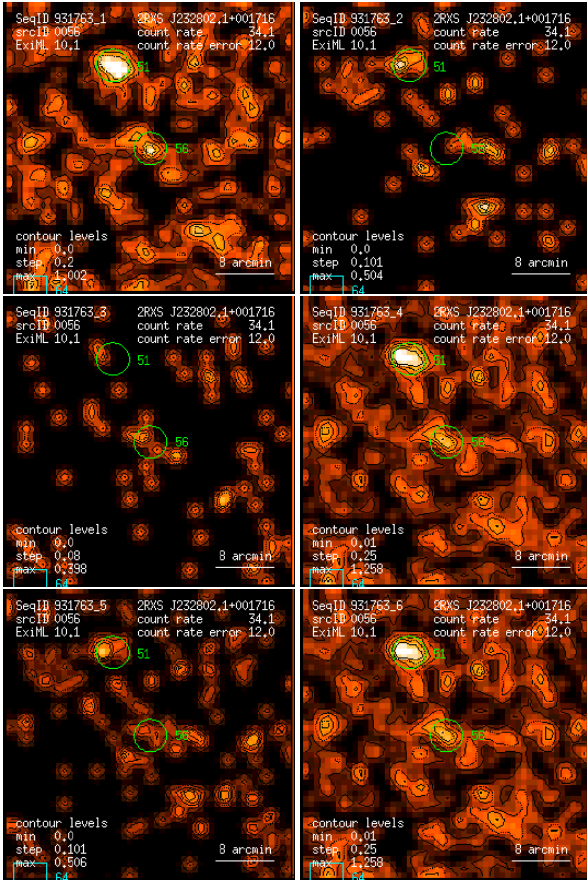
Figure 56: RASS 931763: detection 0056: band rate images, Gaussian filter: (1) PSPC channels 11 – 41, (2) 52 – 90, (3) 91 – 201, (4) 11 – 235, (5) 52 – 201, (6) 11 – 201. Broad band rates in counts/ks. Band rate contour levels in counts/ks/arcmin 2 .
