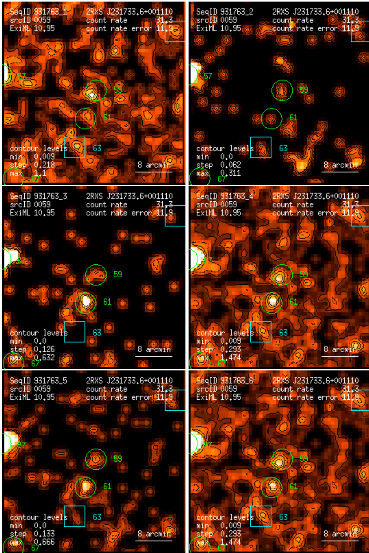
Figure 59: RASS 931763: detection 0059: band rate images, Gaussian filter: (1) PSPC channels 11 – 41, (2) 52 – 90, (3) 91 – 201, (4) 11 – 235, (5) 52 – 201, (6) 11 – 201. Broad band rates in counts/ks. Band rate contour levels in counts/ks/arcmin 2 .
