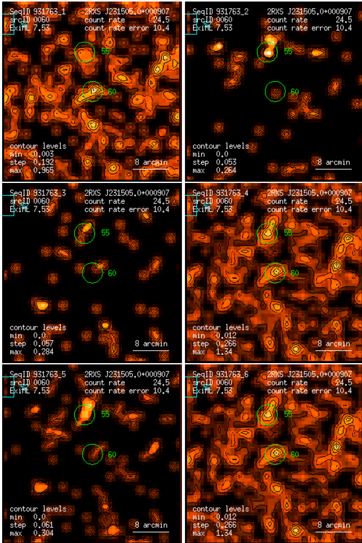
Figure 60: RASS 931763: detection 0060: band rate images, Gaussian filter: (1) PSPC channels 11 – 41, (2) 52 – 90, (3) 91 – 201, (4) 11 – 235, (5) 52 – 201, (6) 11 – 201. Broad band rates in counts/ks. Band rate contour levels in counts/ks/arcmin 2 .
