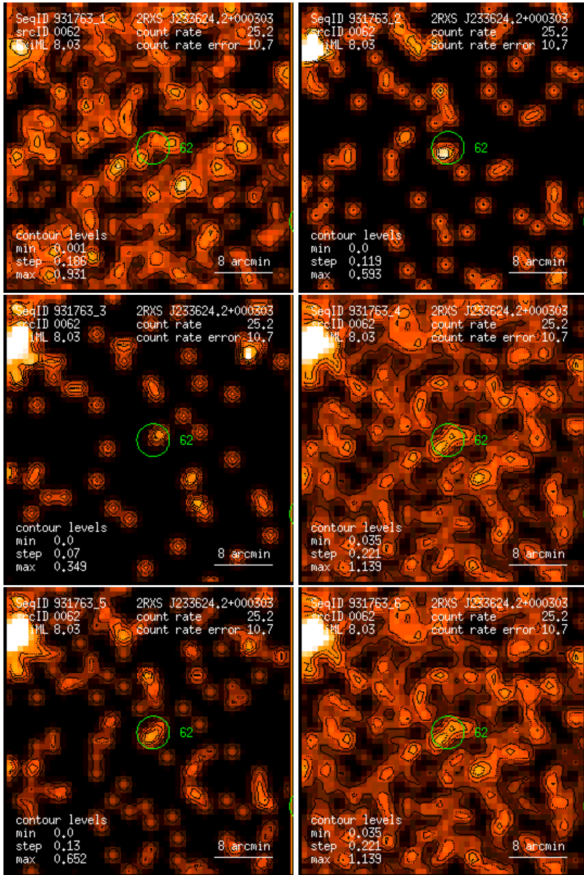
Figure 62: RASS 931763: detection 0062: band rate images, Gaussian filter: (1) PSPC channels 11 – 41, (2) 52 – 90, (3) 91 – 201, (4) 11 – 235, (5) 52 – 201, (6) 11 – 201. Broad band rates in counts/ks. Band rate contour levels in counts/ks/arcmin 2 .
