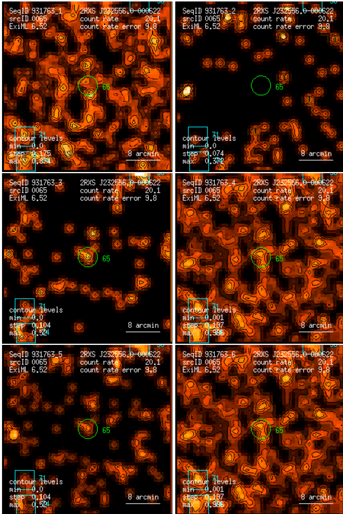
Figure 65: RASS 931763: detection 0065: band rate images, Gaussian filter: (1) PSPC channels 11 – 41, (2) 52 – 90, (3) 91 – 201, (4) 11 – 235, (5) 52 – 201, (6) 11 – 201. Broad band rates in counts/ks. Band rate contour levels in counts/ks/arcmin 2 .
