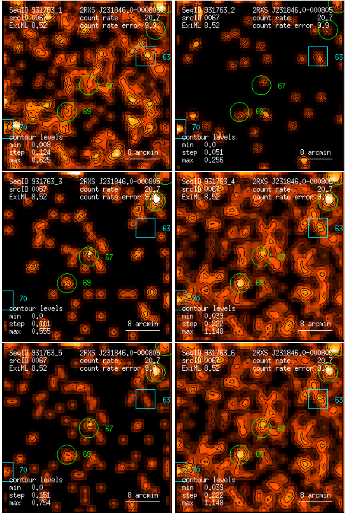
Figure 67: RASS 931763: detection 0067: band rate images, Gaussian filter: (1) PSPC channels 11 – 41, (2) 52 – 90, (3) 91 – 201, (4) 11 – 235, (5) 52 – 201, (6) 11 – 201. Broad band rates in counts/ks. Band rate contour levels in counts/ks/arcmin 2 .
