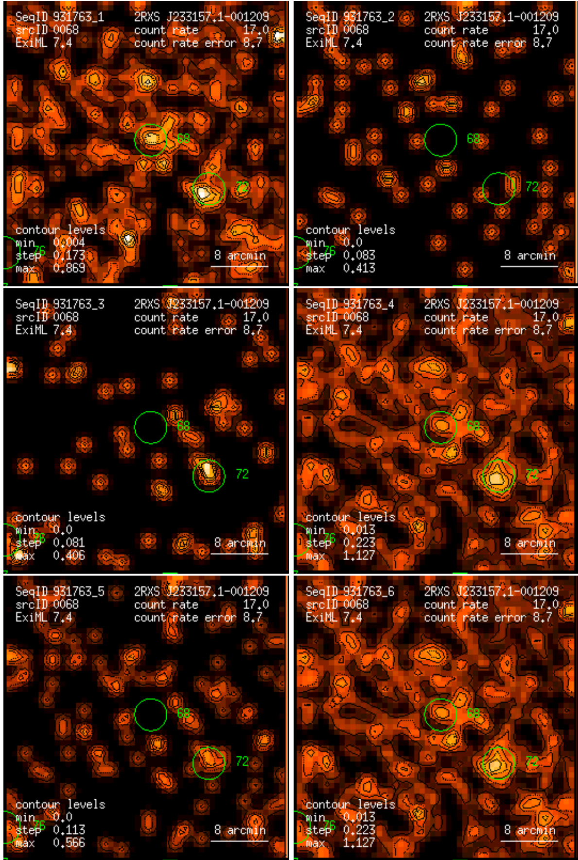
Figure 68: RASS 931763: detection 0068: band rate images, Gaussian filter: (1) PSPC channels 11 – 41, (2) 52 – 90, (3) 91 – 201, (4) 11 – 235, (5) 52 – 201, (6) 11 – 201. Broad band rates in counts/ks. Band rate contour levels in counts/ks/arcmin 2 .
