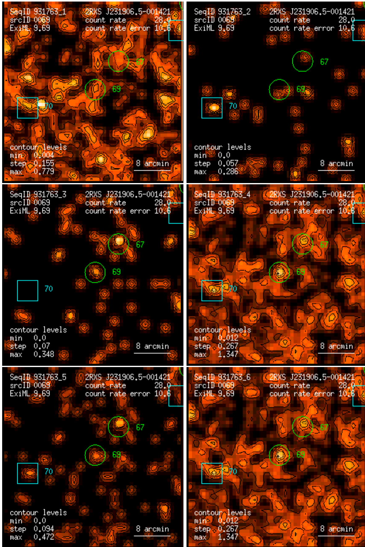
Figure 69: RASS 931763: detection 0069: band rate images, Gaussian filter: (1) PSPC channels 11 – 41, (2) 52 – 90, (3) 91 – 201, (4) 11 – 235, (5) 52 – 201, (6) 11 – 201. Broad band rates in counts/ks. Band rate contour levels in counts/ks/arcmin 2 .
