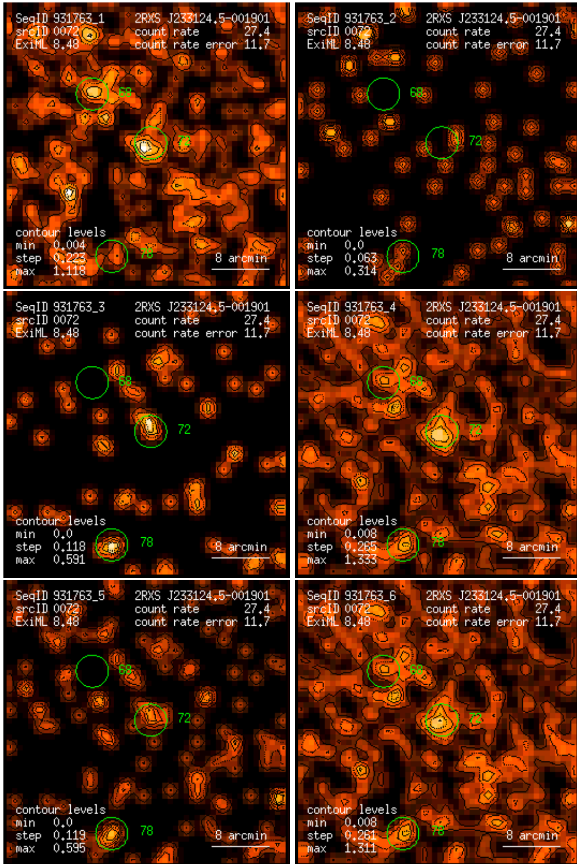
Figure 72: RASS 931763: detection 0072: band rate images, Gaussian filter: (1) PSPC channels 11 – 41, (2) 52 – 90, (3) 91 – 201, (4) 11 – 235, (5) 52 – 201, (6) 11 – 201. Broad band rates in counts/ks. Band rate contour levels in counts/ks/arcmin 2 .
