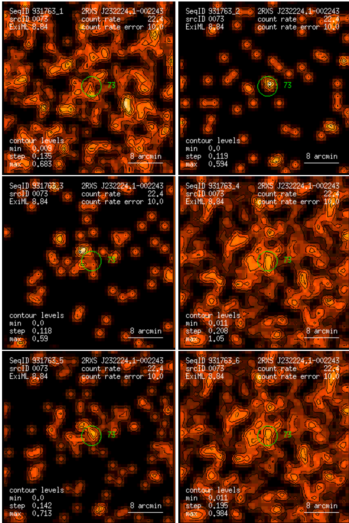
Figure 73: RASS 931763: detection 0073: band rate images, Gaussian filter: (1) PSPC channels 11 – 41, (2) 52 – 90, (3) 91 – 201, (4) 11 – 235, (5) 52 – 201, (6) 11 – 201. Broad band rates in counts/ks. Band rate contour levels in counts/ks/arcmin 2 .
