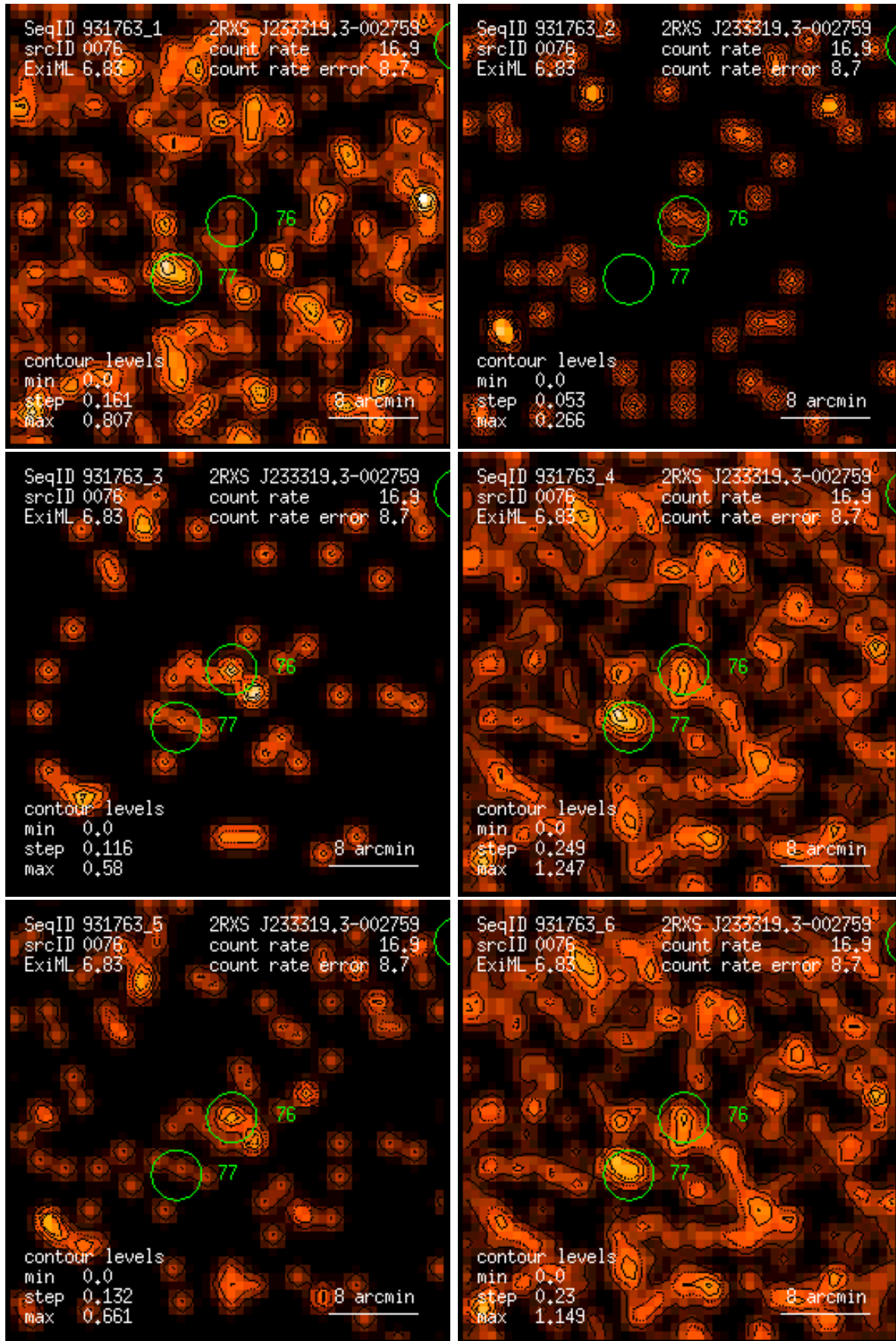
Figure 76: RASS 931763: detection 0076: band rate images, Gaussian filter: (1) PSPC channels 11 – 41, (2) 52 – 90, (3) 91 – 201, (4) 11 – 235, (5) 52 – 201, (6) 11 – 201. Broad band rates in counts/ks. Band rate contour levels in counts/ks/arcmin 2 .
