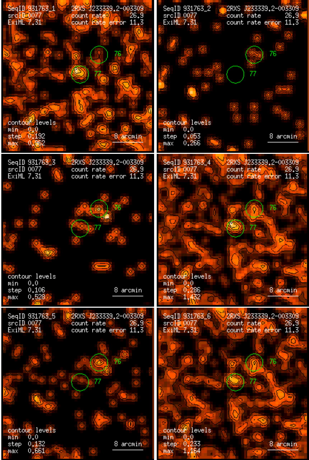
Figure 77: RASS 931763: detection 0077: band rate images, Gaussian filter: (1) PSPC channels 11 – 41, (2) 52 – 90, (3) 91 – 201, (4) 11 – 235, (5) 52 – 201, (6) 11 – 201. Broad band rates in counts/ks. Band rate contour levels in counts/ks/arcmin 2 .
