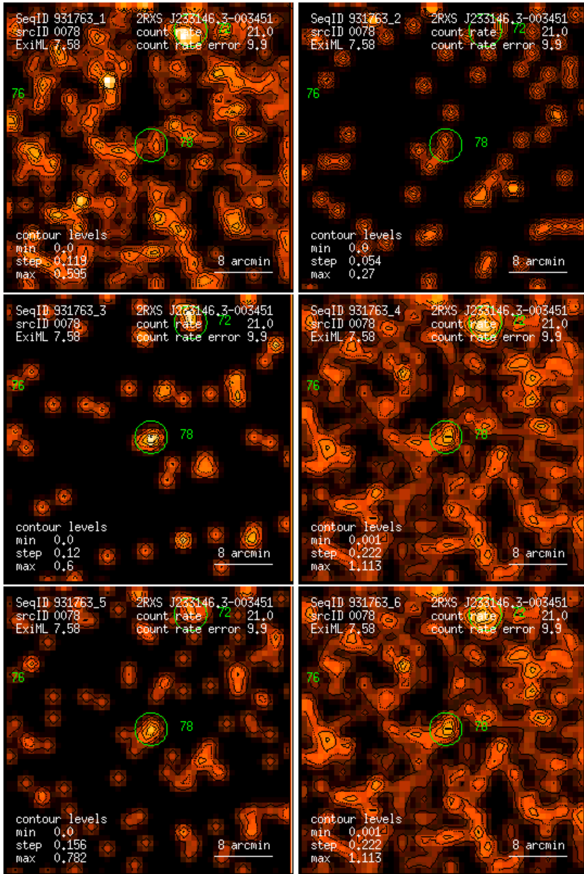
Figure 78: RASS 931763: detection 0078: band rate images, Gaussian filter: (1) PSPC channels 11 – 41, (2) 52 – 90, (3) 91 – 201, (4) 11 – 235, (5) 52 – 201, (6) 11 – 201. Broad band rates in counts/ks. Band rate contour levels in counts/ks/arcmin 2 .
