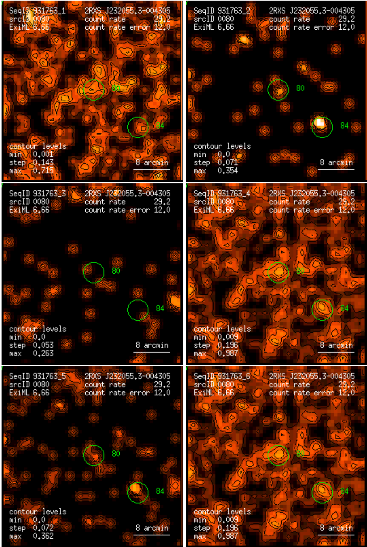
Figure 80: RASS 931763: detection 0080: band rate images, Gaussian filter: (1) PSPC channels 11 – 41, (2) 52 – 90, (3) 91 – 201, (4) 11 – 235, (5) 52 – 201, (6) 11 – 201. Broad band rates in counts/ks. Band rate contour levels in counts/ks/arcmin 2 .
