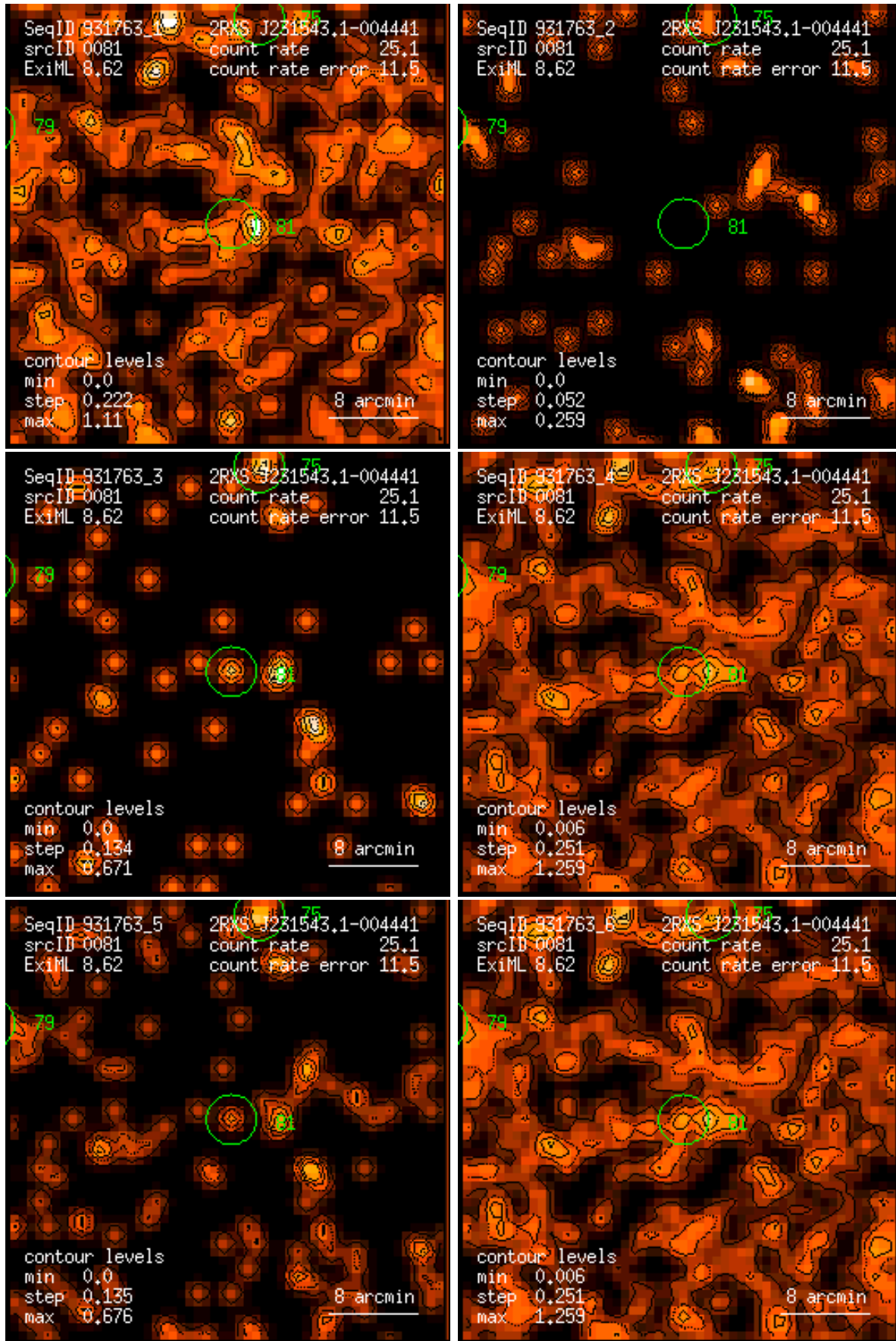
Figure 81: RASS 931763: detection 0081: band rate images, Gaussian filter: (1) PSPC channels 11 – 41, (2) 52 – 90, (3) 91 – 201, (4) 11 – 235, (5) 52 – 201, (6) 11 – 201. Broad band rates in counts/ks. Band rate contour levels in counts/ks/arcmin 2 .
