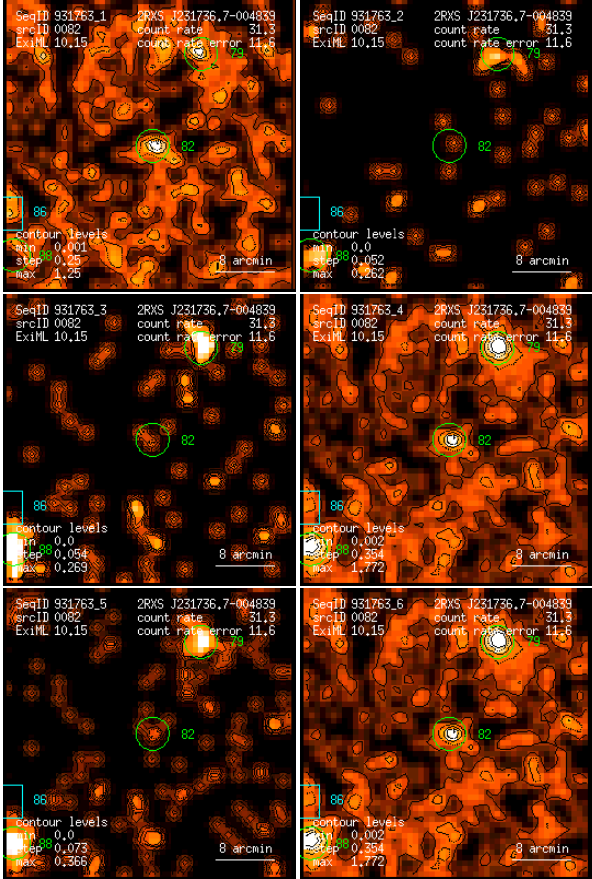
Figure 82: RASS 931763: detection 0082: band rate images, Gaussian filter: (1) PSPC channels 11 – 41, (2) 52 – 90, (3) 91 – 201, (4) 11 – 235, (5) 52 – 201, (6) 11 – 201. Broad band rates in counts/ks. Band rate contour levels in counts/ks/arcmin 2 .
