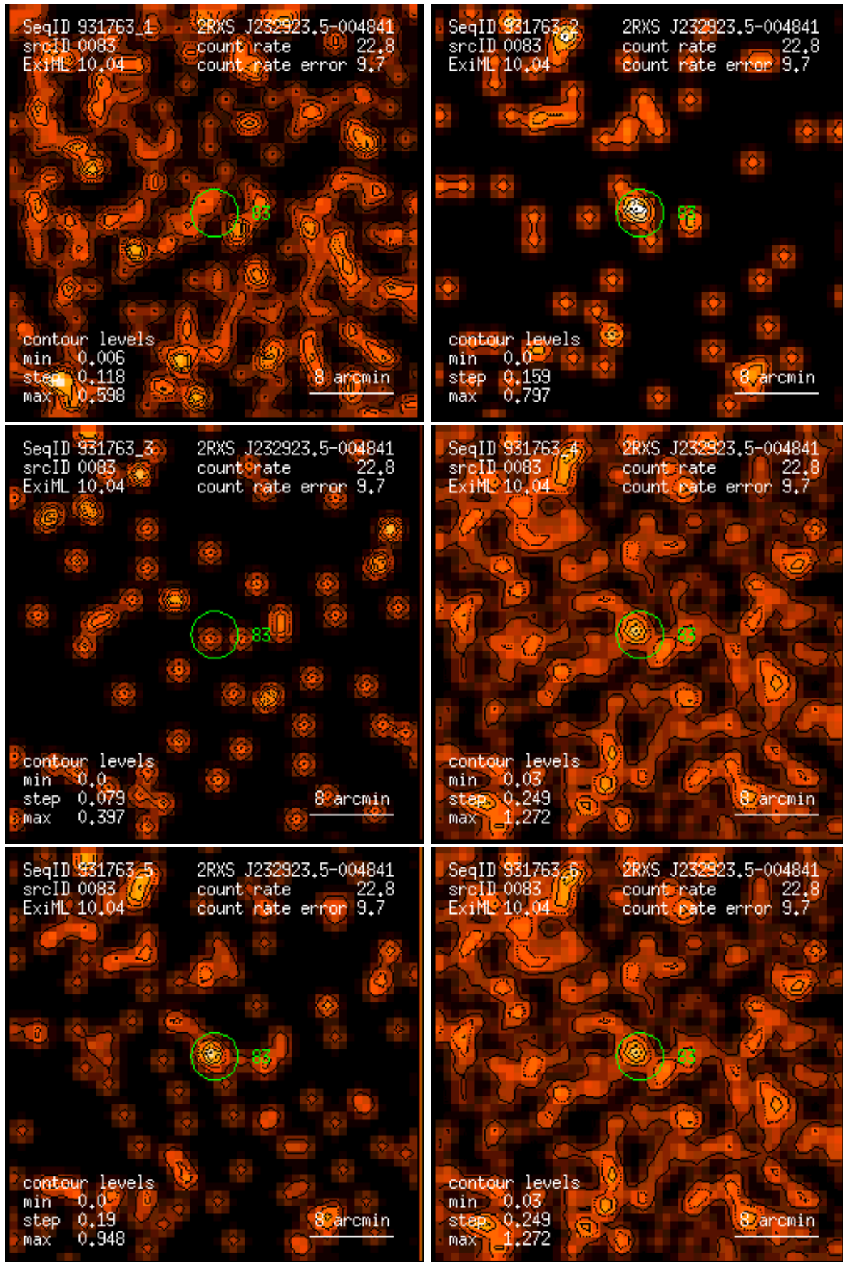
Figure 83: RASS 931763: detection 0083: band rate images, Gaussian filter: (1) PSPC channels 11 – 41, (2) 52 – 90, (3) 91 – 201, (4) 11 – 235, (5) 52 – 201, (6) 11 – 201. Broad band rates in counts/ks. Band rate contour levels in counts/ks/arcmin 2 .
