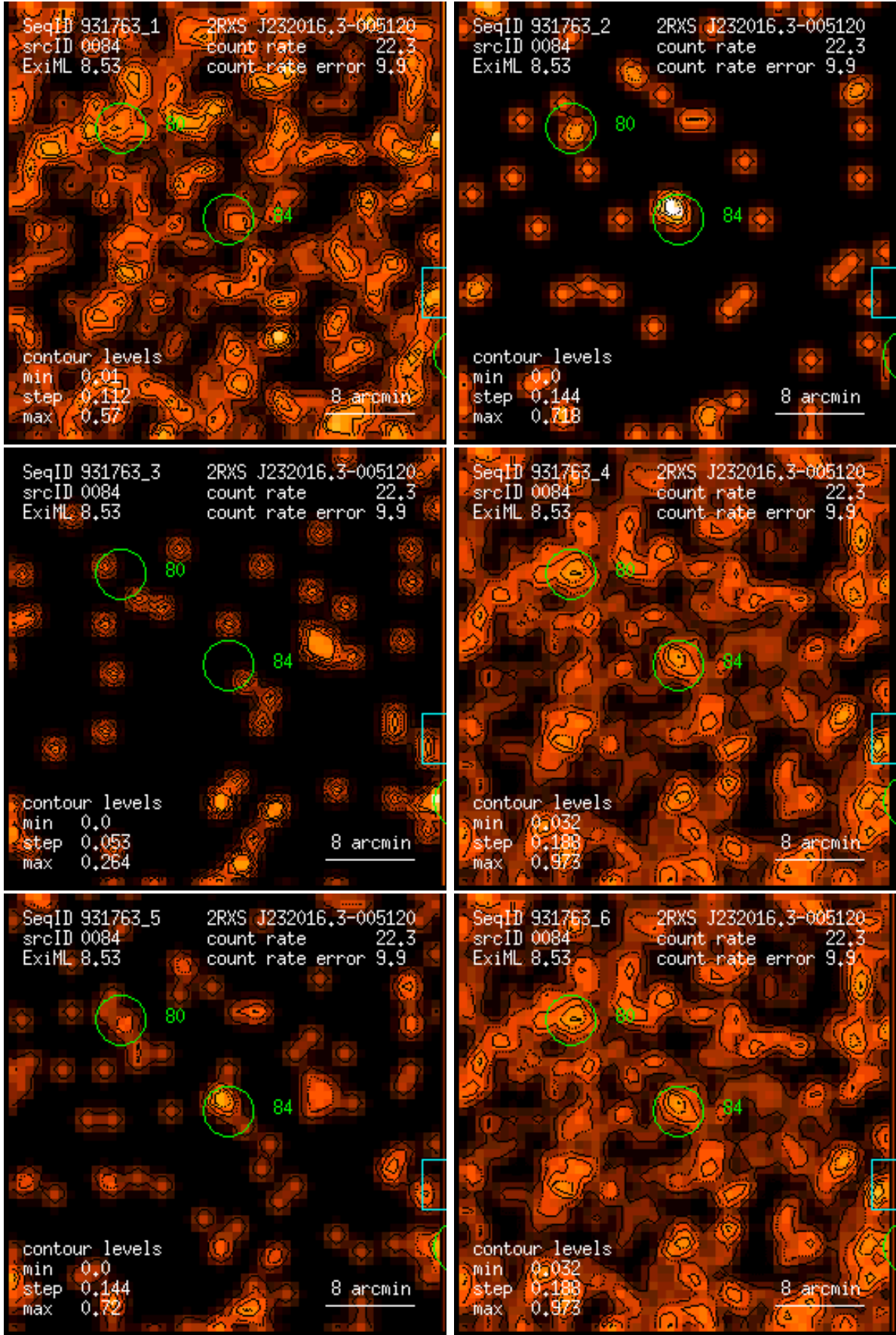
Figure 84: RASS 931763: detection 0084: band rate images, Gaussian filter: (1) PSPC channels 11 – 41, (2) 52 – 90, (3) 91 – 201, (4) 11 – 235, (5) 52 – 201, (6) 11 – 201. Broad band rates in counts/ks. Band rate contour levels in counts/ks/arcmin 2 .
