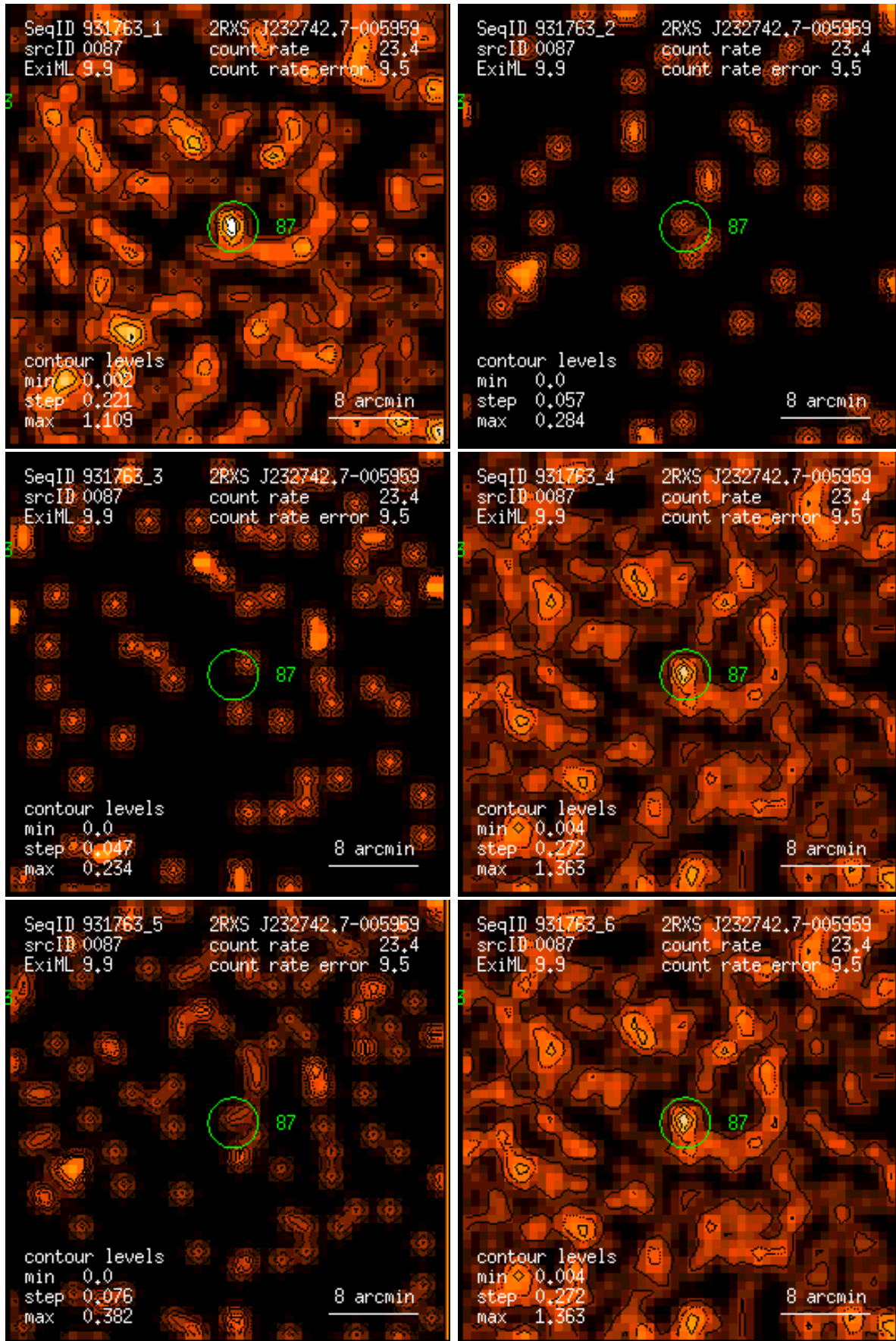
Figure 87: RASS 931763: detection 0087: band rate images, Gaussian filter: (1) PSPC channels 11 – 41, (2) 52 – 90, (3) 91 – 201, (4) 11 – 235, (5) 52 – 201, (6) 11 – 201. Broad band rates in counts/ks. Band rate contour levels in counts/ks/arcmin 2 .
