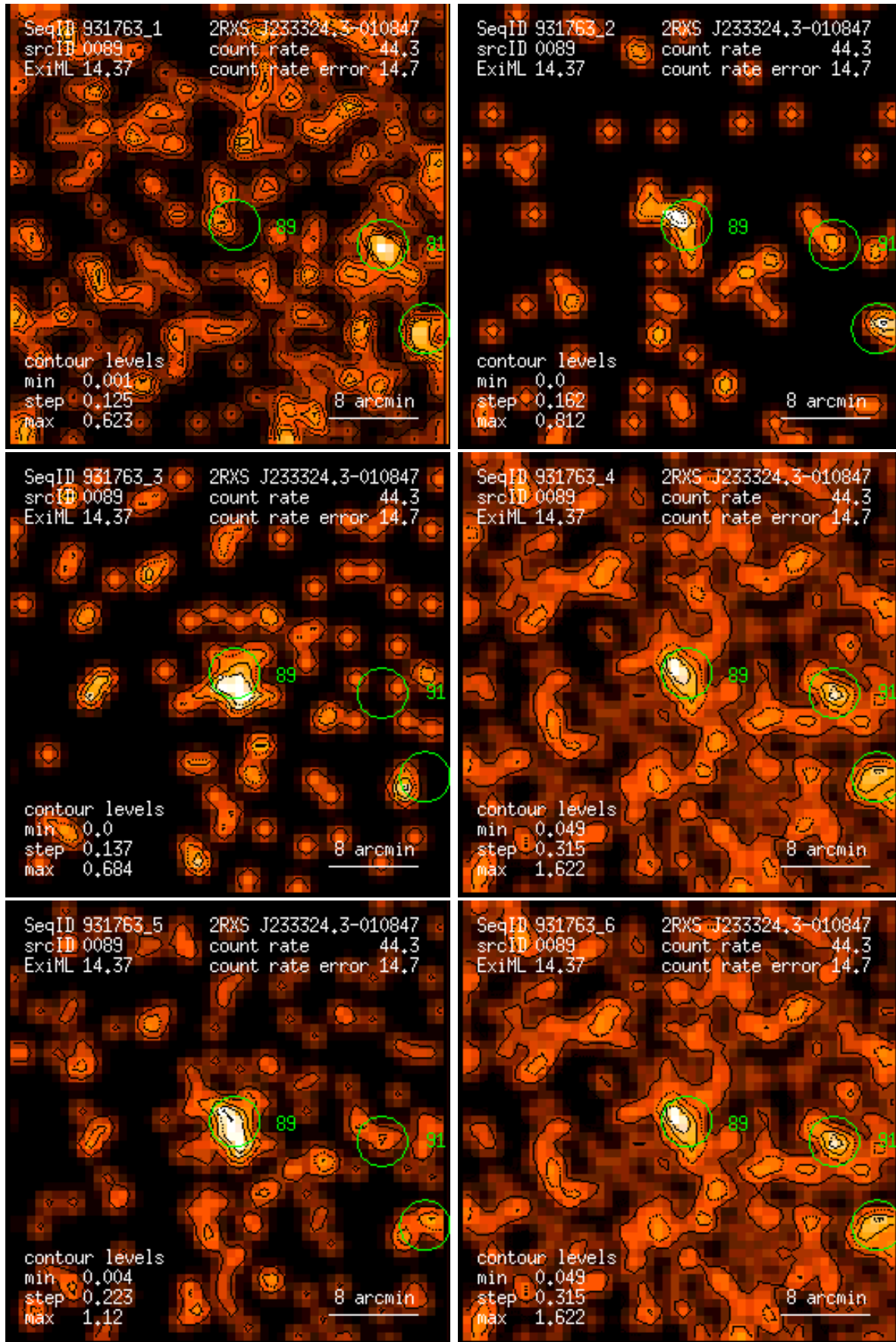
Figure 89: RASS 931763: detection 0089: band rate images, Gaussian filter: (1) PSPC channels 11 – 41, (2) 52 – 90, (3) 91 – 201, (4) 11 – 235, (5) 52 – 201, (6) 11 – 201. Broad band rates in counts/ks. Band rate contour levels in counts/ks/arcmin 2 .
